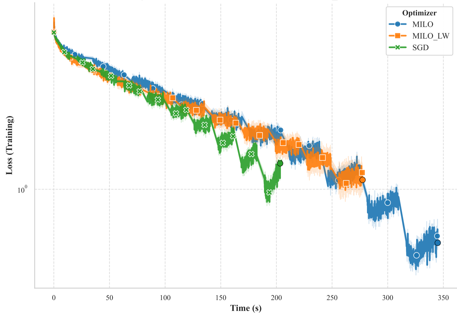
Training Loss vs. Wall-clock Time for RESNET34_CIFAR100
