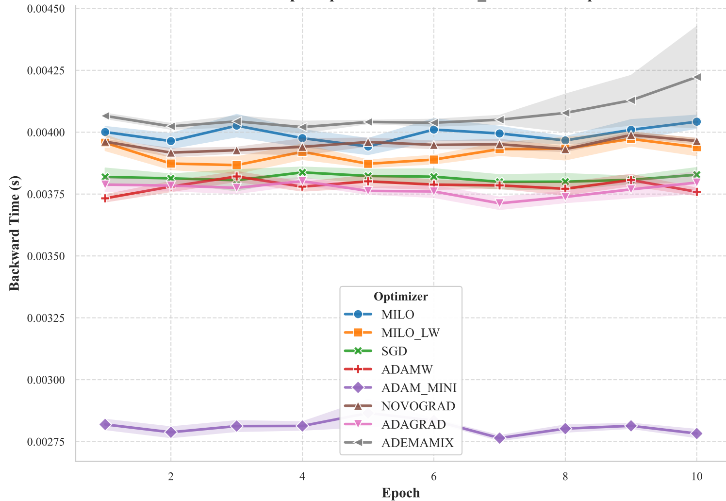
Backward Runtime per Epoch for RESNET34_CIFAR100 Experiment
