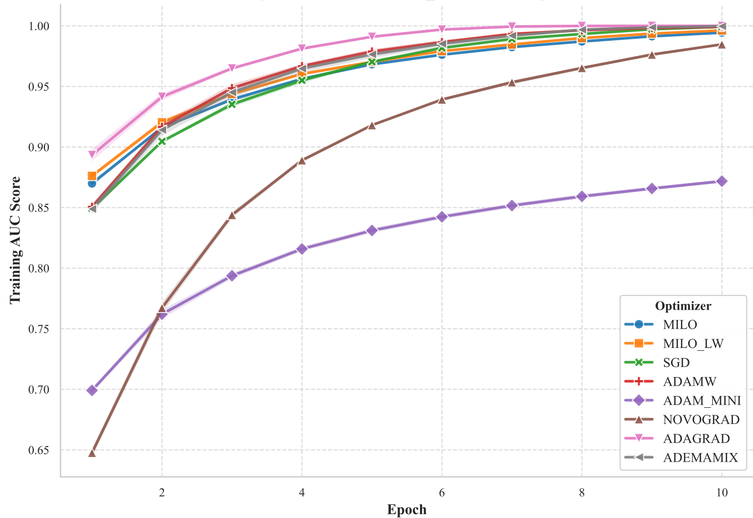
Training AUC for RESNET34_CIFAR100 Experiment
