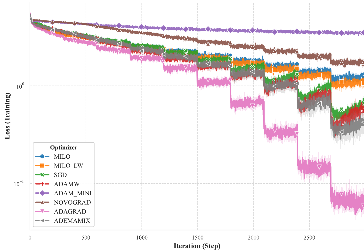
Training Loss vs. Iteration for RESNET34_CIFAR100 Experiment
