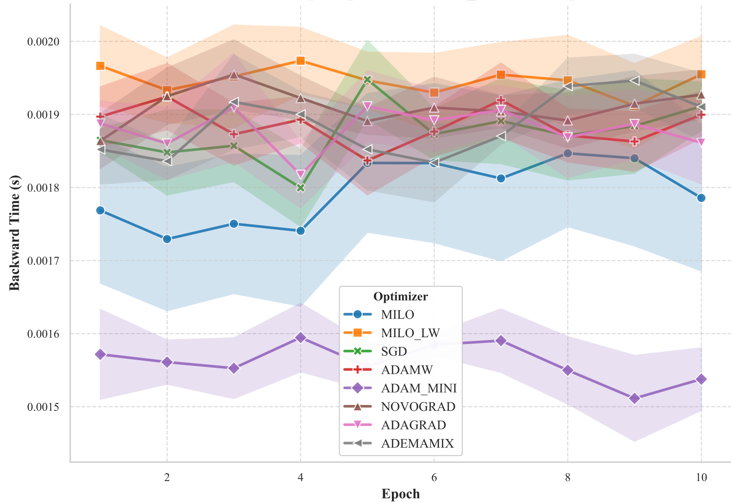
Backward Runtime per Epoch for VGG11_CIFAR10 Experiment
