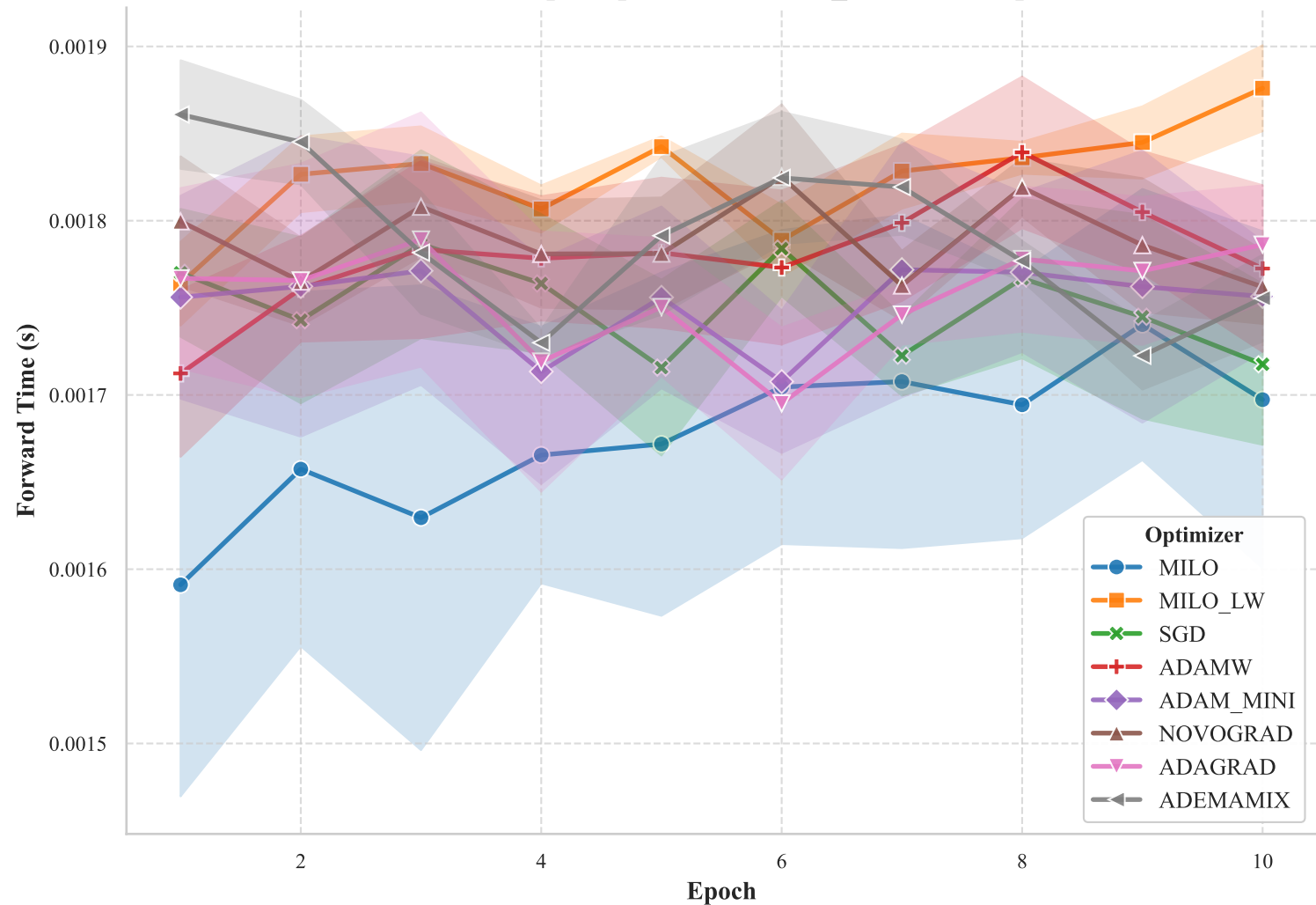
Forward Runtime per Epoch for VGG11_CIFAR10 Experiment
