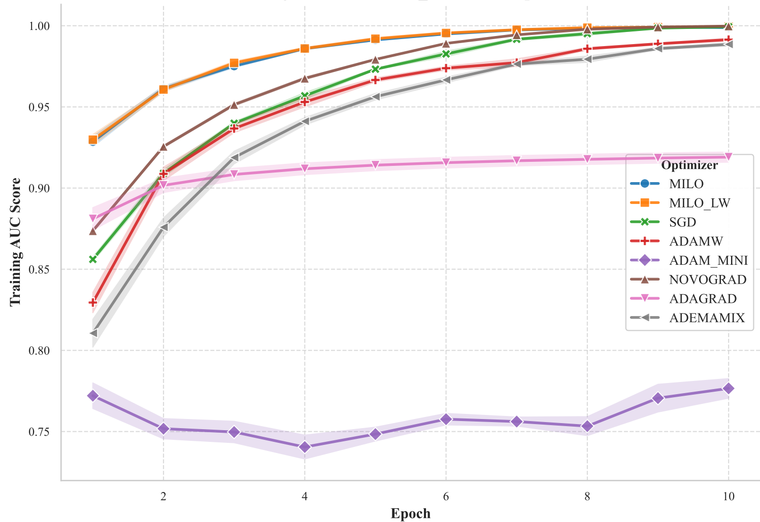
Training AUC for VGG11_CIFAR10 Experiment
