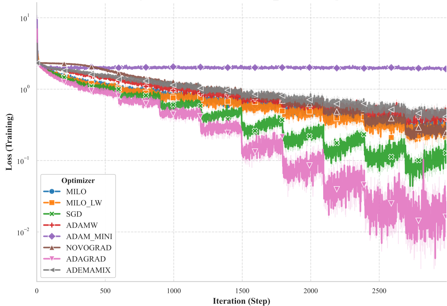
Training Loss vs. Iteration for VGG11_CIFAR10 Experiment
