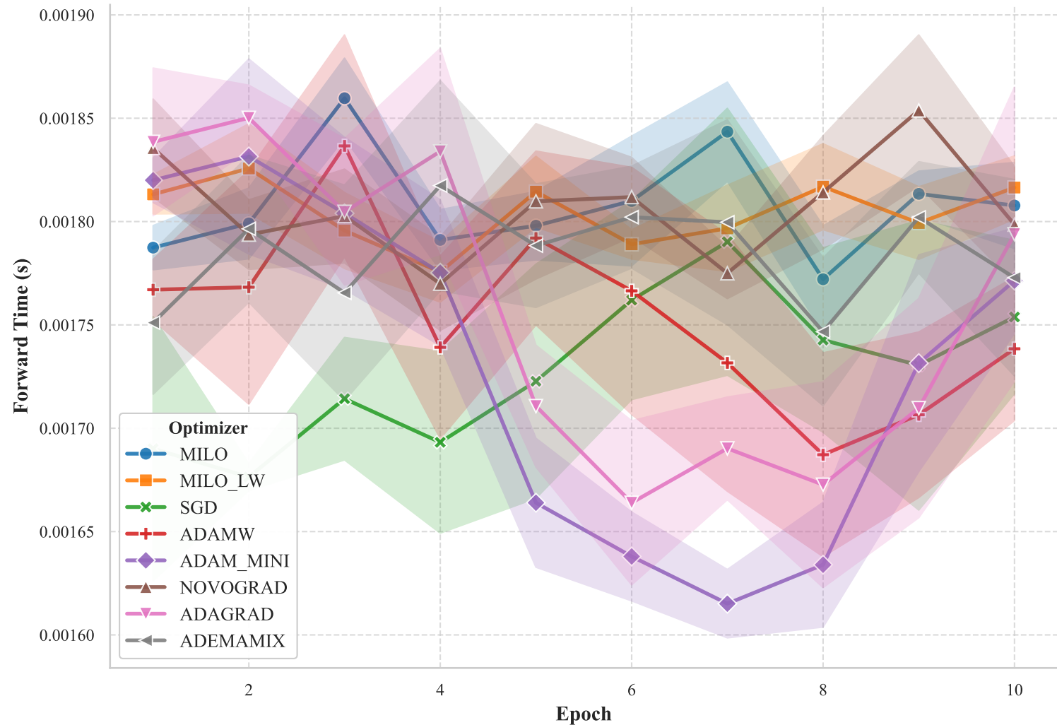
Forward Runtime per Epoch for VGG11_CIFAR100 Experiment
