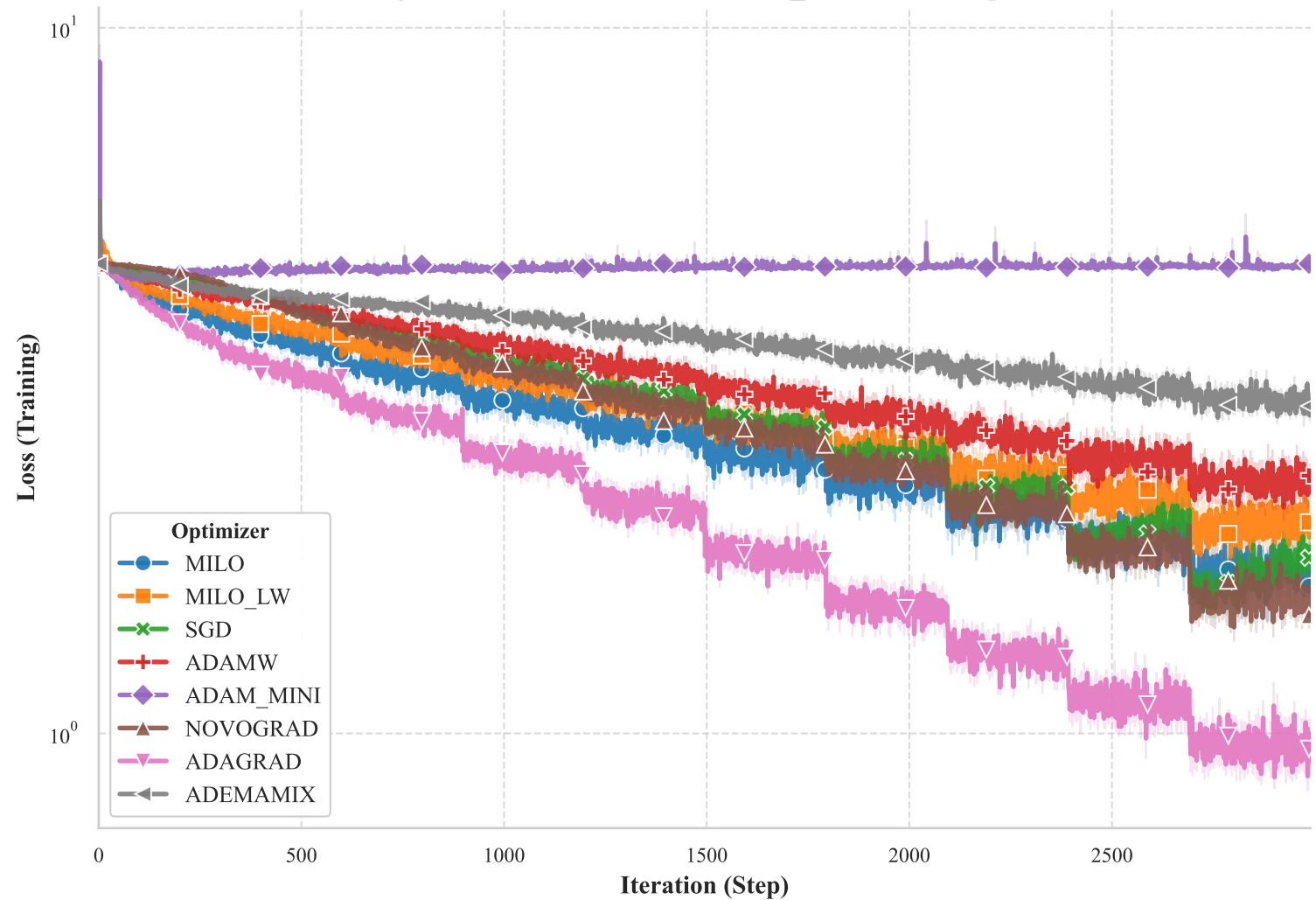
Training Loss vs. Iteration for VGG11_CIFAR100 Experiment
