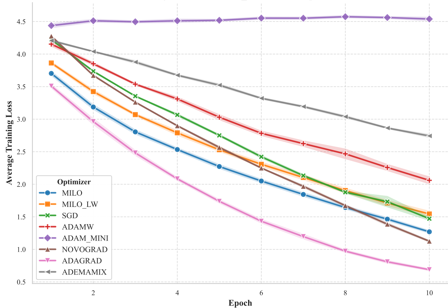
Training Loss for VGG11_CIFAR100 Experiment
