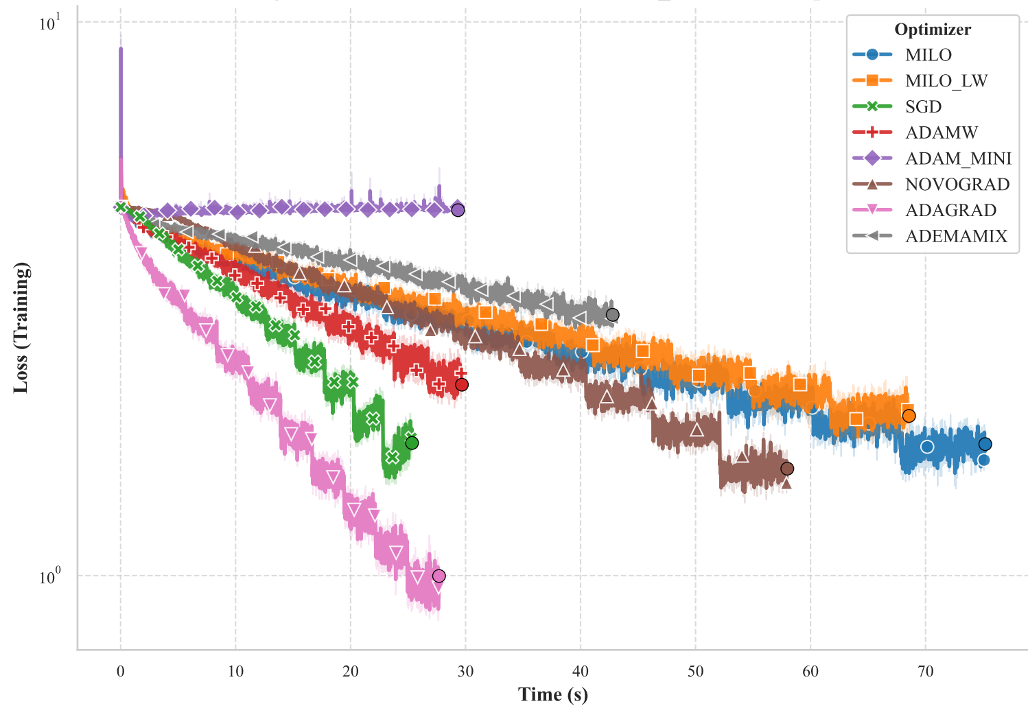
Training Loss vs. Wall-clock Time for VGG11_CIFAR100 Experiment
