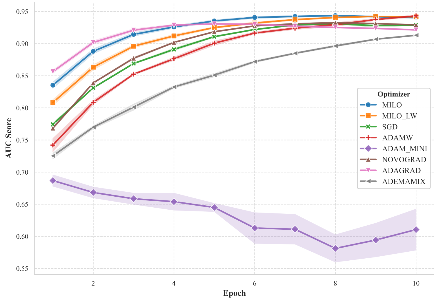
Validation AUC for VGG11_CIFAR100 Experiment
