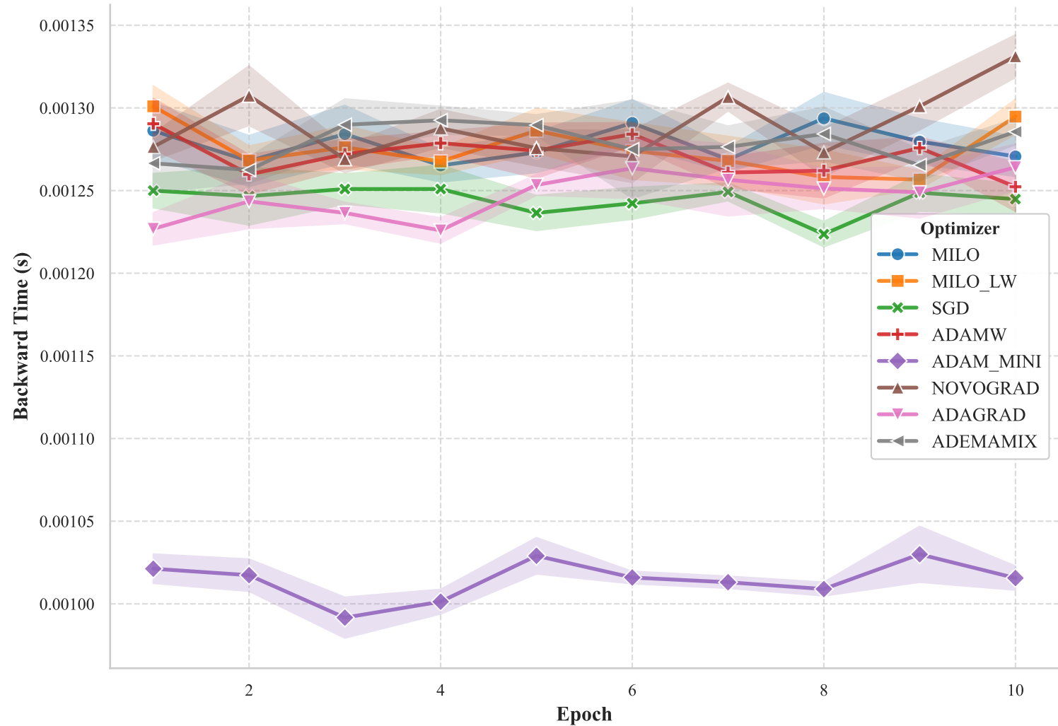
Backward Runtime per Epoch for VGG11_CIFAR100 Experiment
