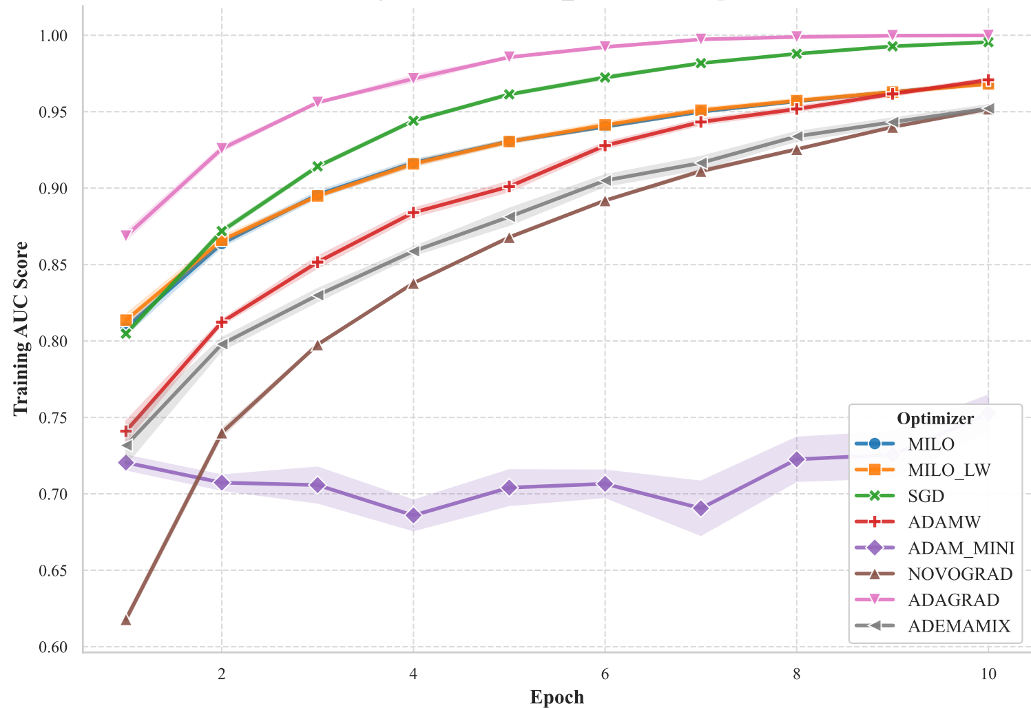
Training AUC for VGG11_CIFAR100 Experiment
