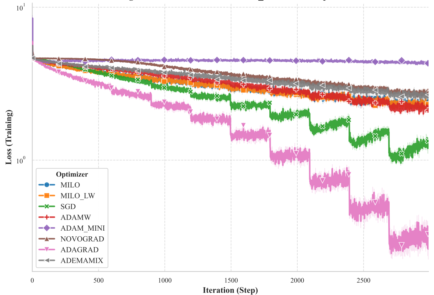
Training Loss vs. Iteration for VGG11_CIFAR100 Experiment
