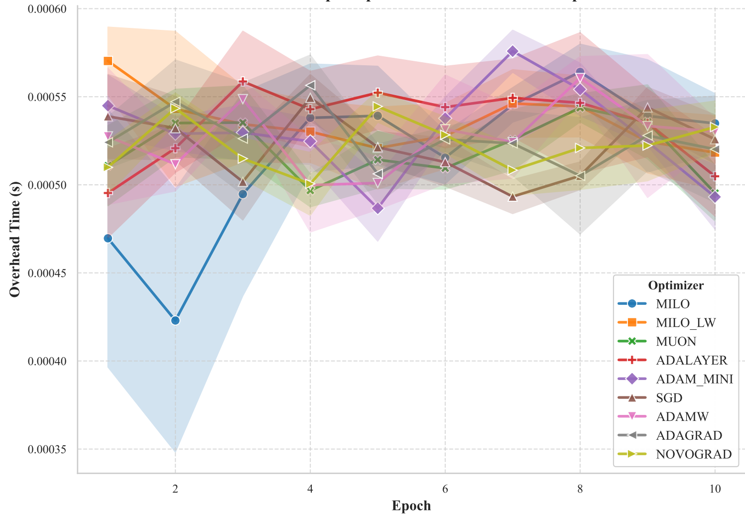
Overhead Runtime per Epoch for MULTILAYER Experiment
