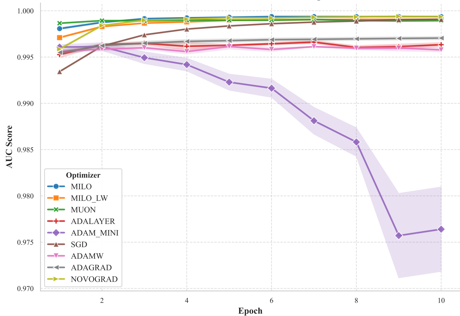
Validation AUC for MULTILAYER Experiment
