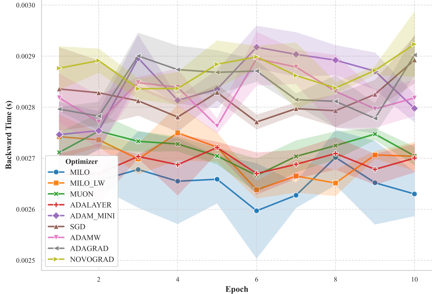
Backward Runtime per Epoch for RESNET18 Experiment
