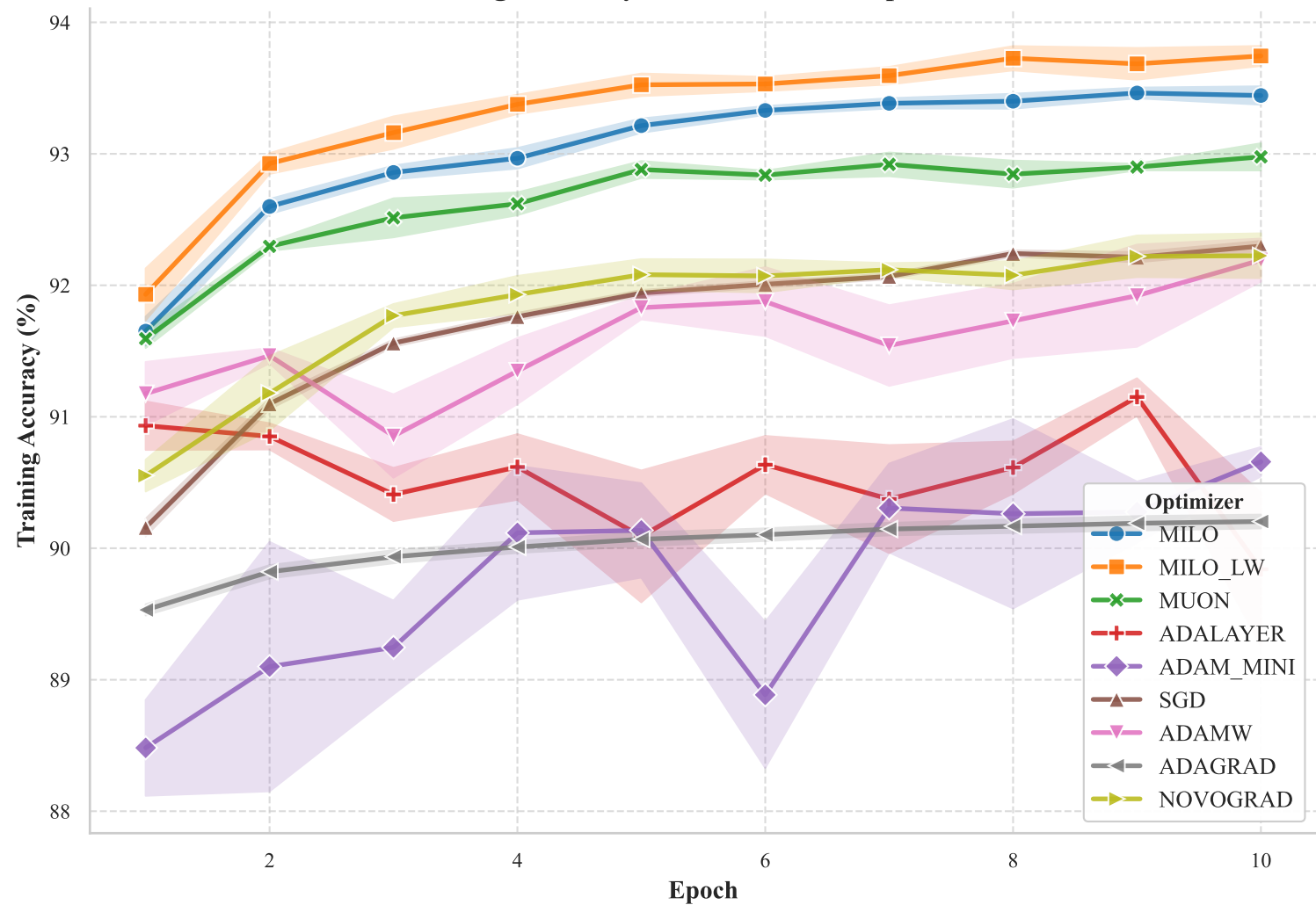
Training Accuracy for LOGISTIC Experiment
