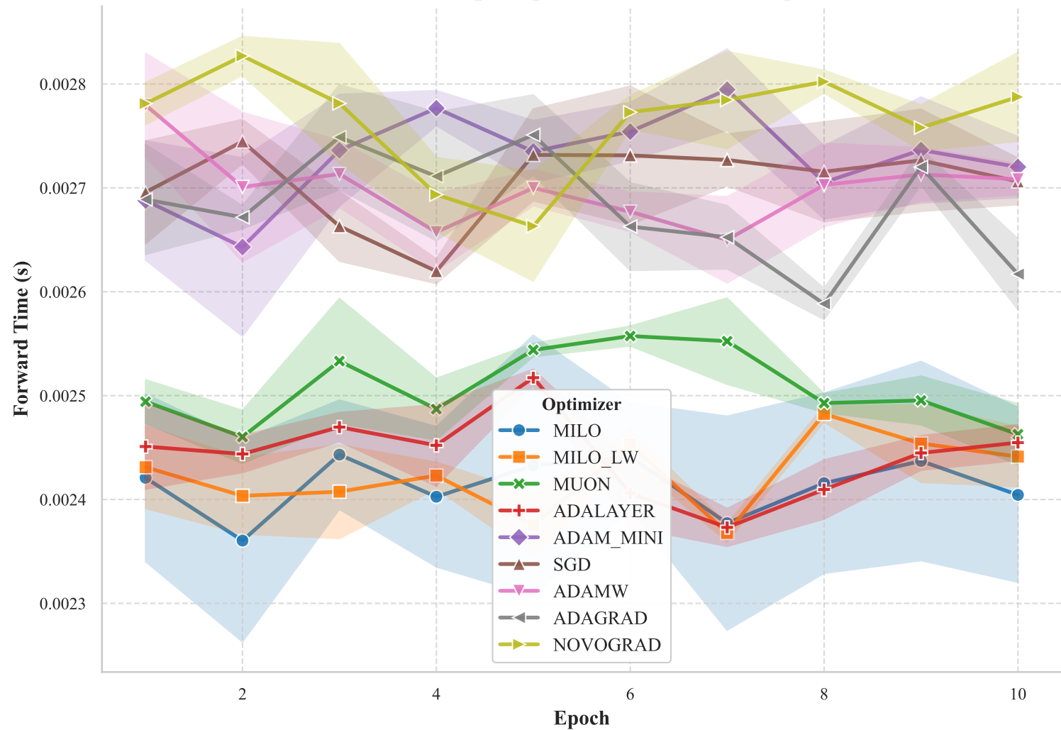
Forward Runtime per Epoch for RESNET18 Experiment
