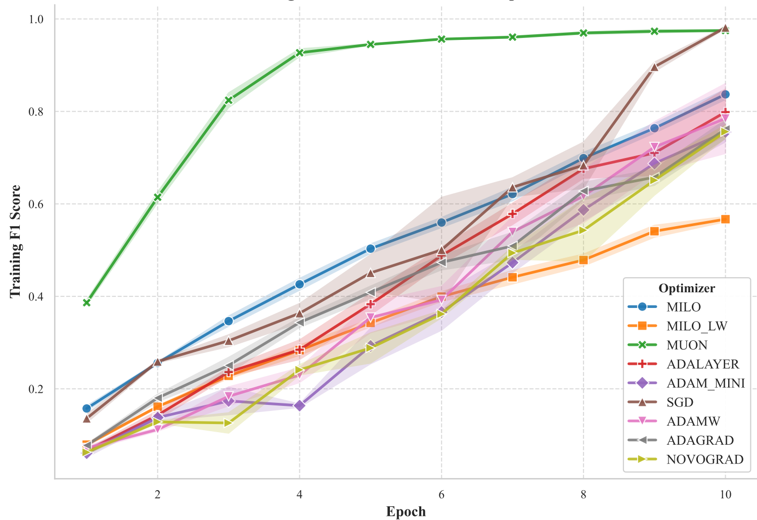
Training F1 Score for RESNET18 Experiment
