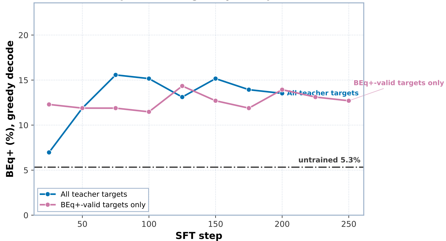
Statement equivalence (greedy T=0, paired, n=244)
