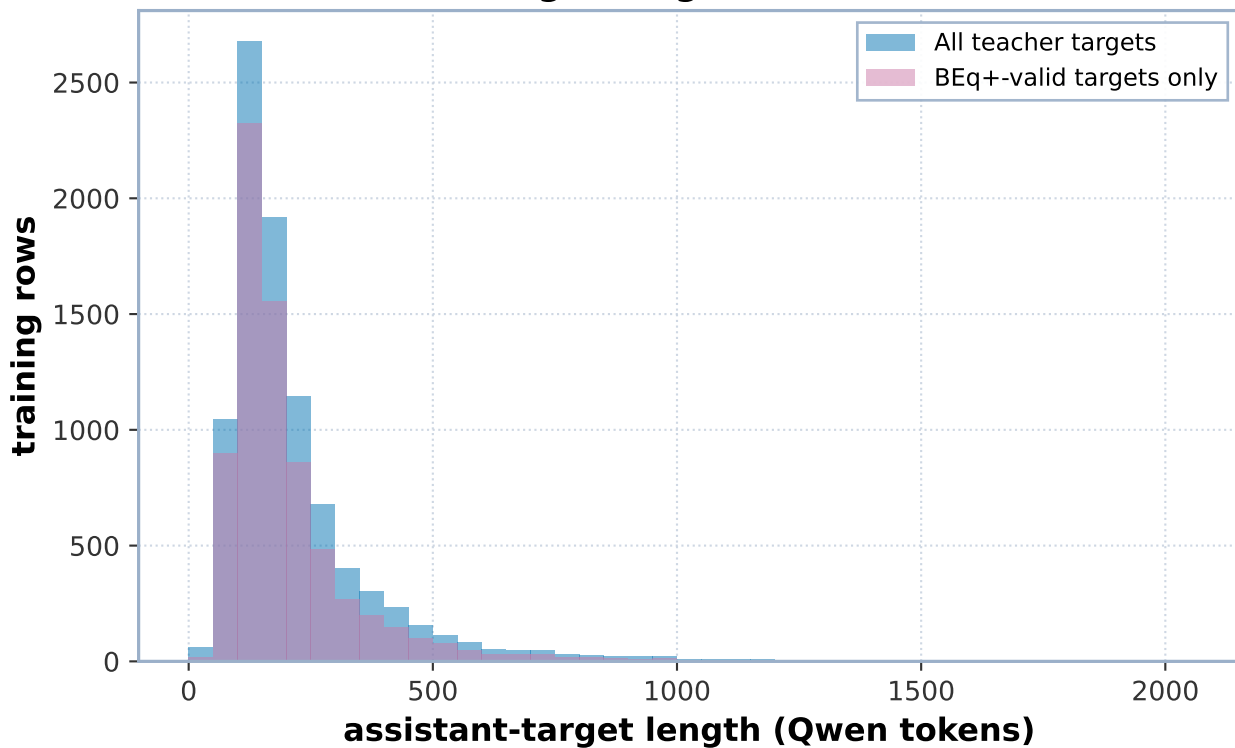
SFT target length distribution
