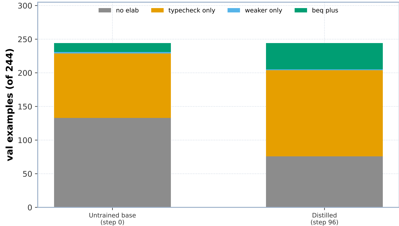
Outcome breakdown at best checkpoint
