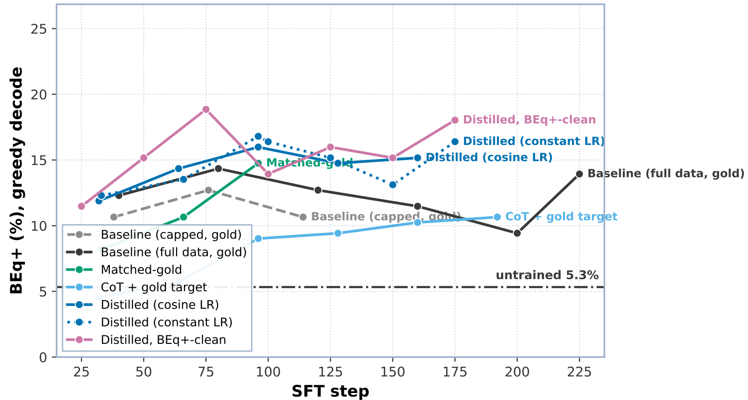
Statement equivalence (greedy T=0, paired, n=244)
