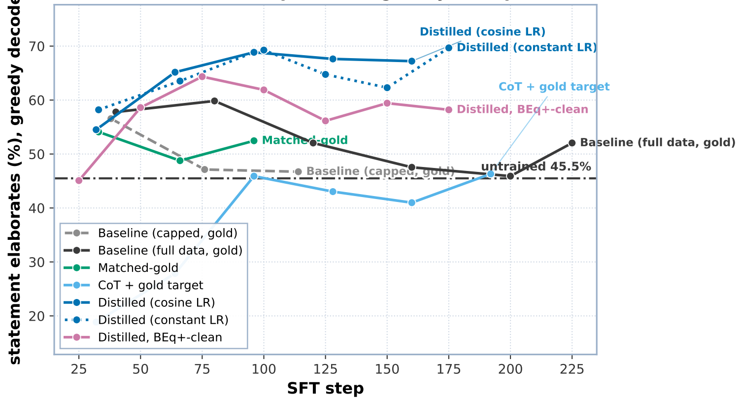
Statement elaboration rate (pass@1) (greedy T=0, paired, n=244)
