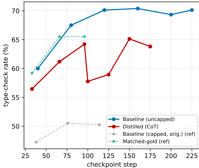
type-check rate
