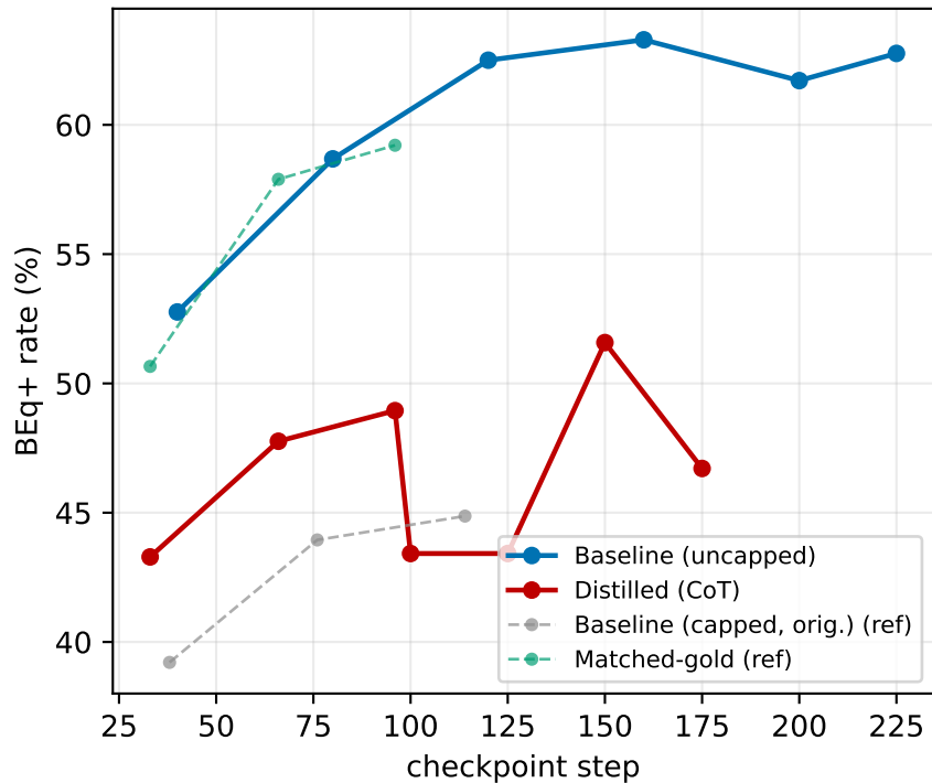
BEq+ rate
