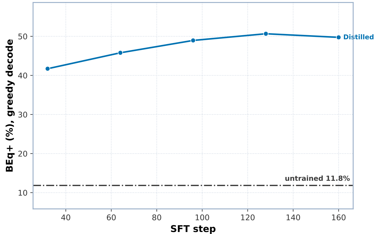
Semantic accuracy (greedy T=0, paired, n=760)
