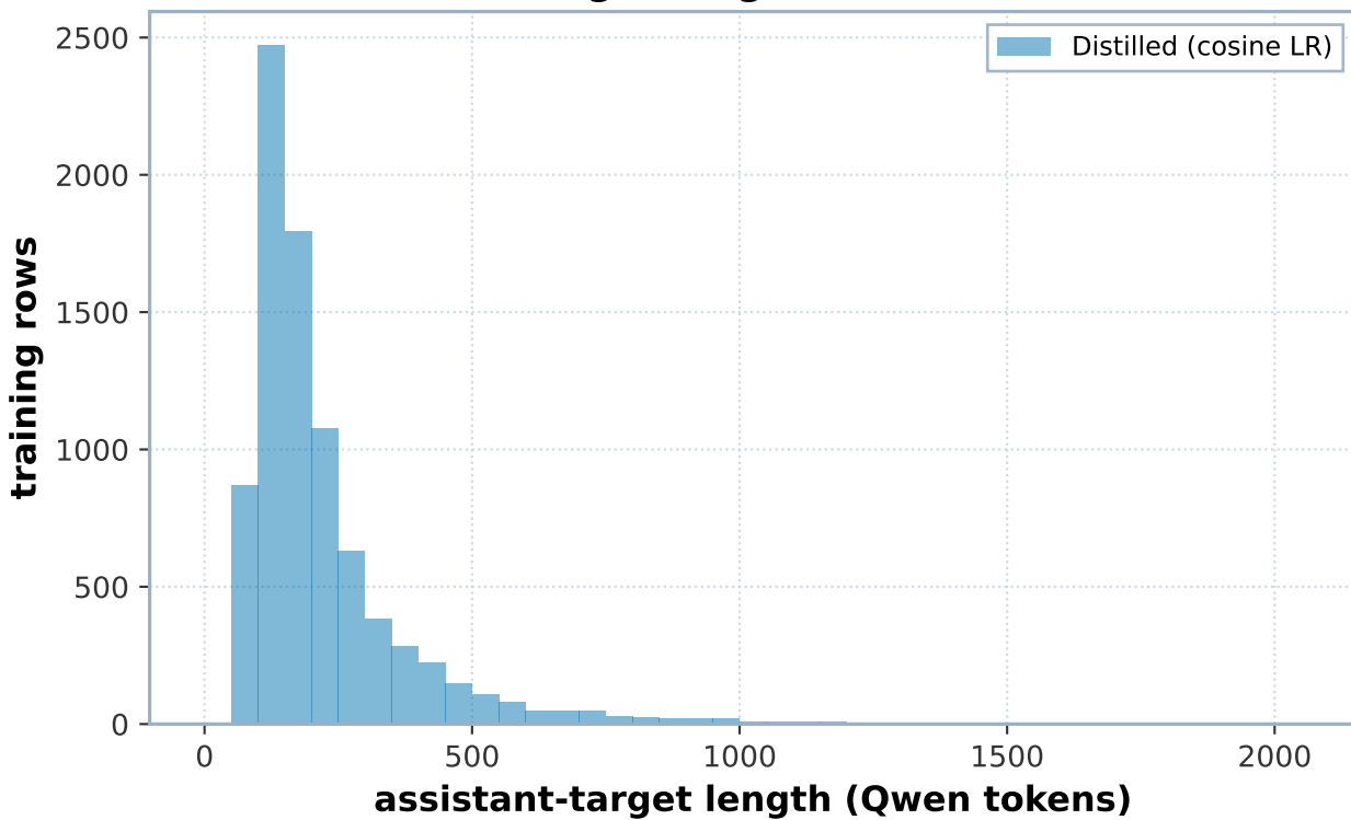
SFT target length distribution
