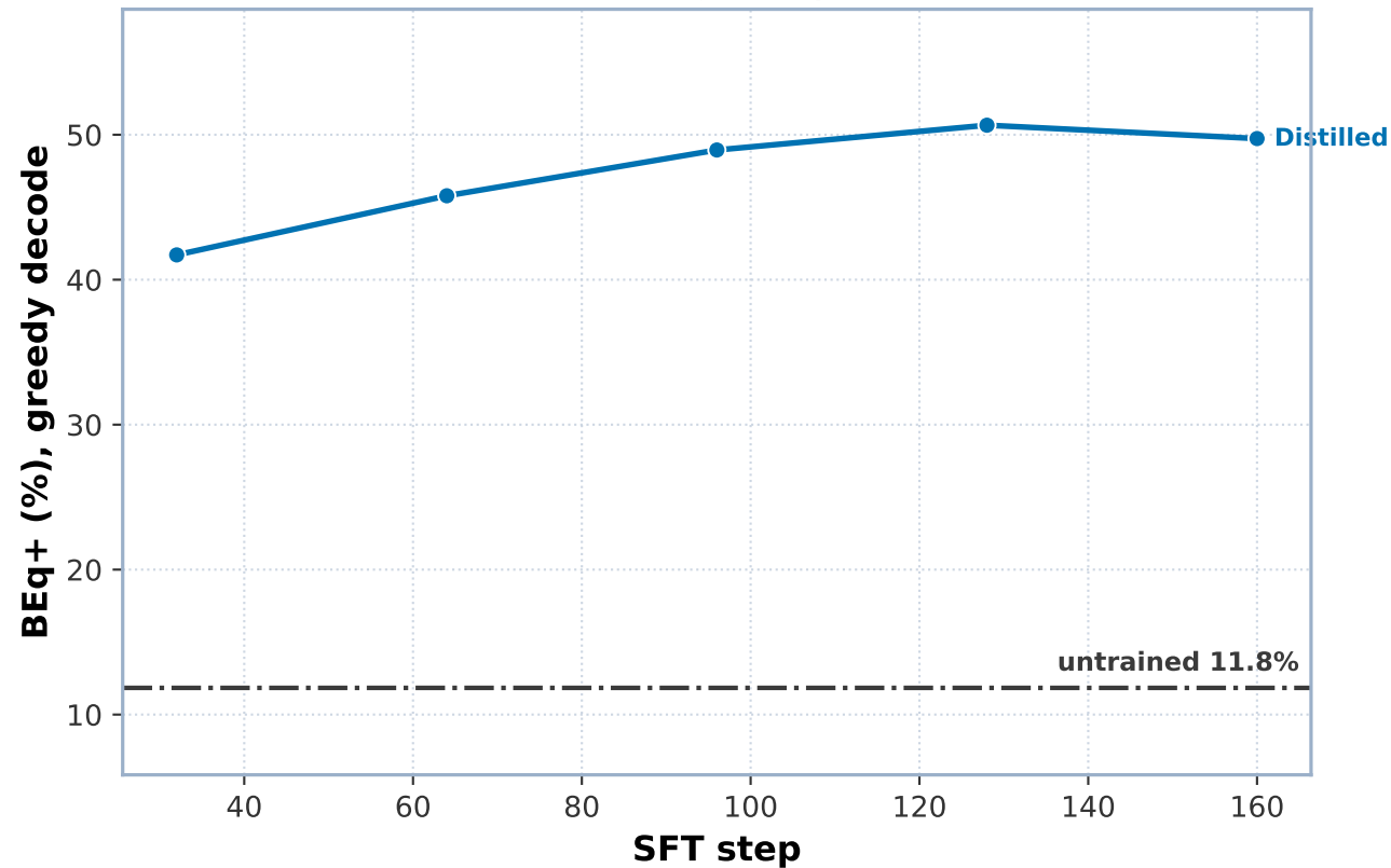
Statement equivalence (greedy T=0, paired, n=760)
