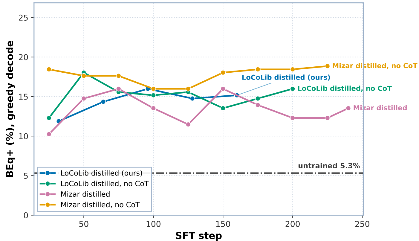
Statement equivalence (greedy T=0, paired, n=244)
