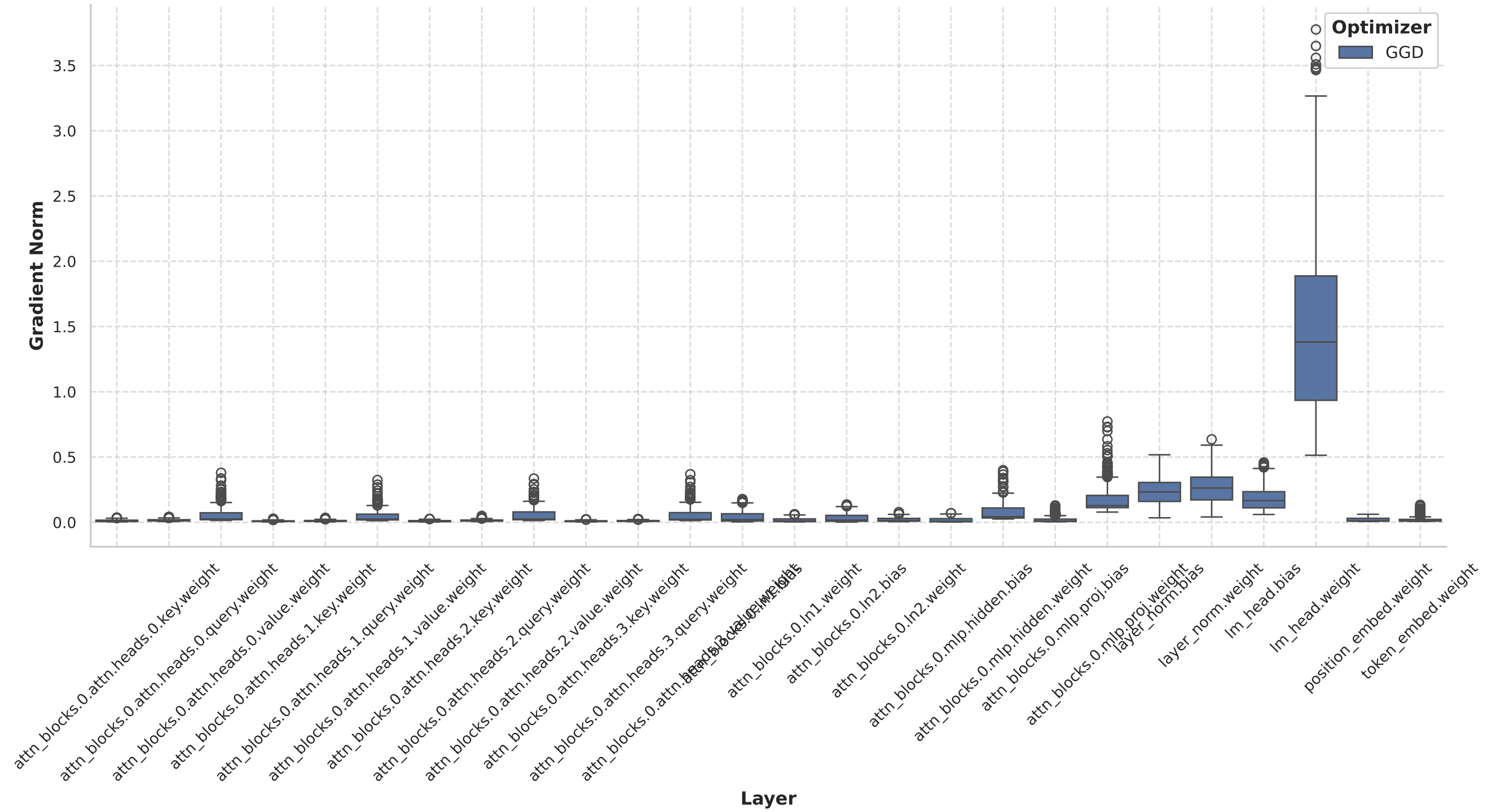
Transformer Training (GGD): Gradient Norm Distribution per Layer
