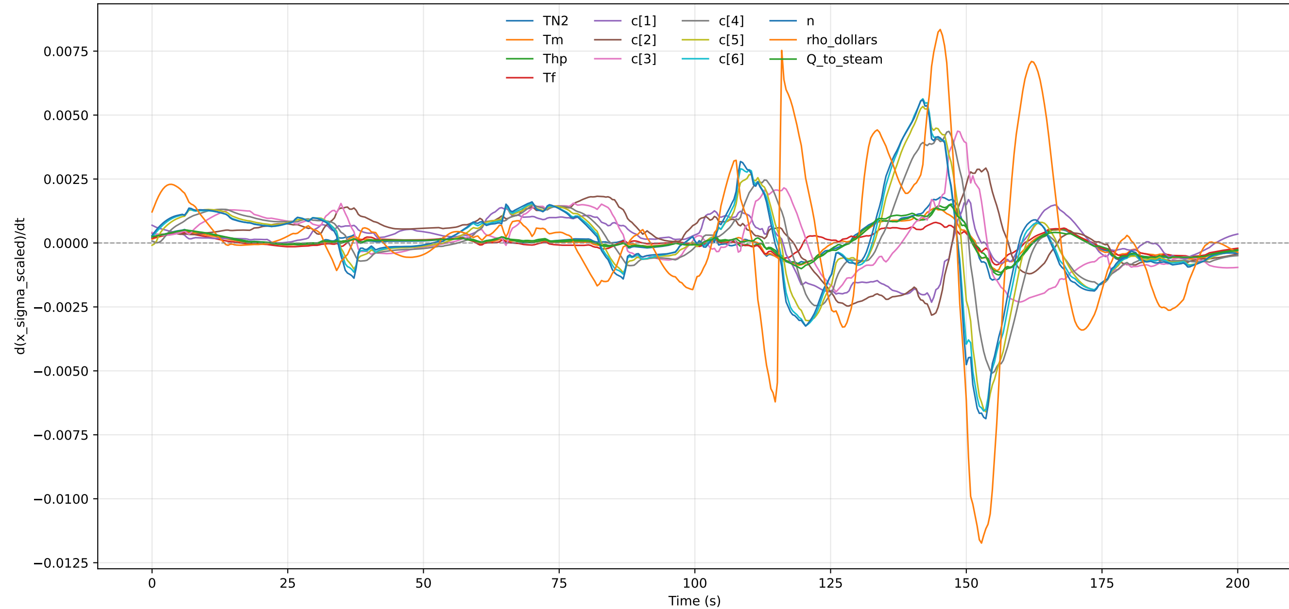
Scaled Uncertainty Derivative - profile_000025
