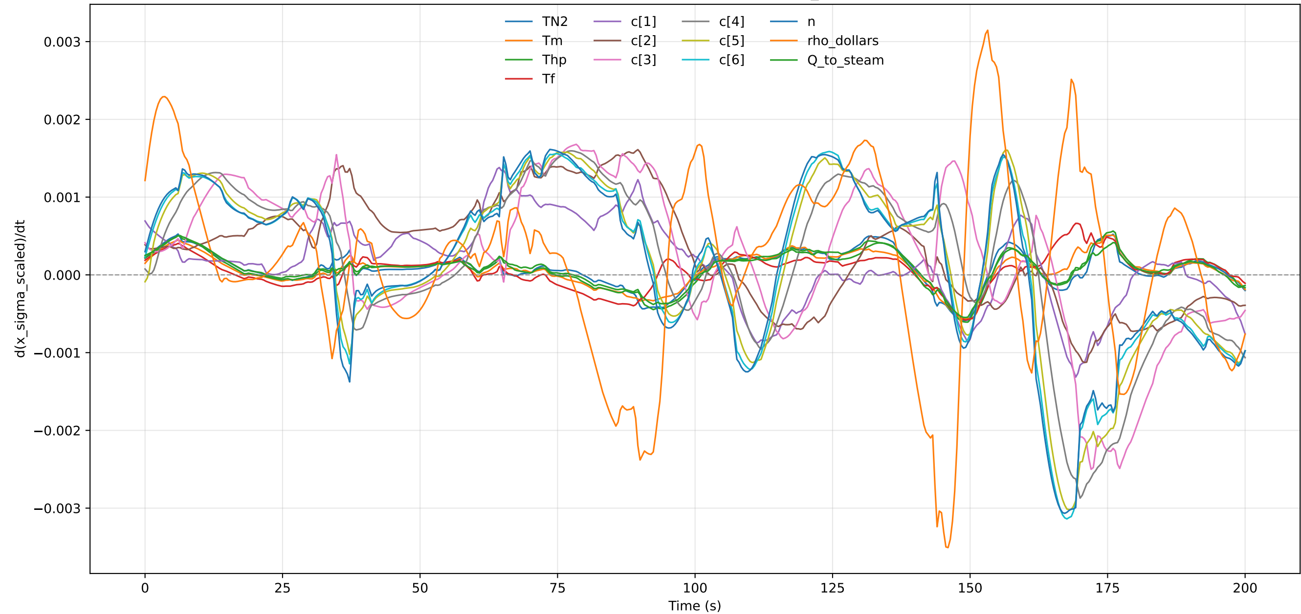
Scaled Uncertainty Derivative - profile_000009
