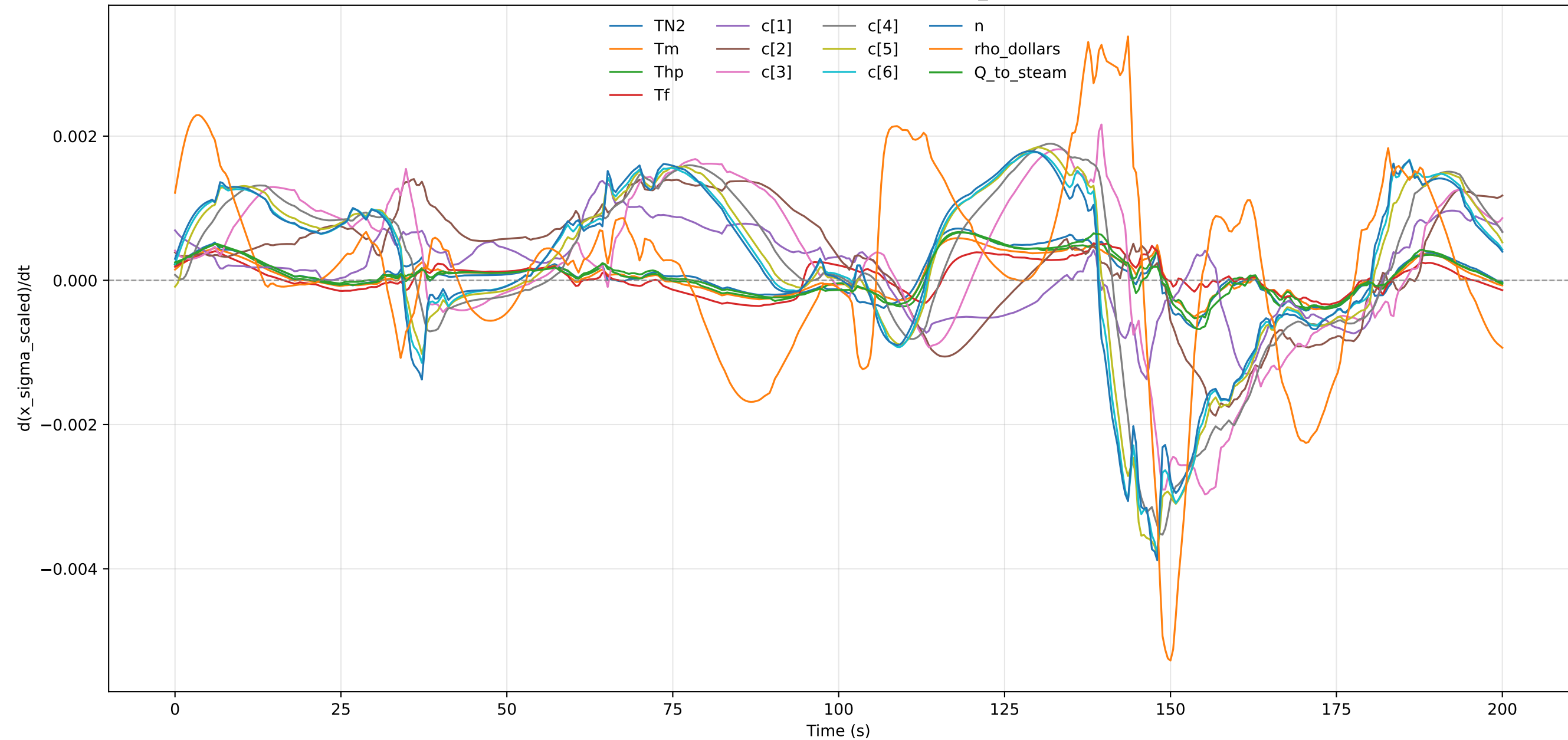
Scaled Uncertainty Derivative - profile_000004
