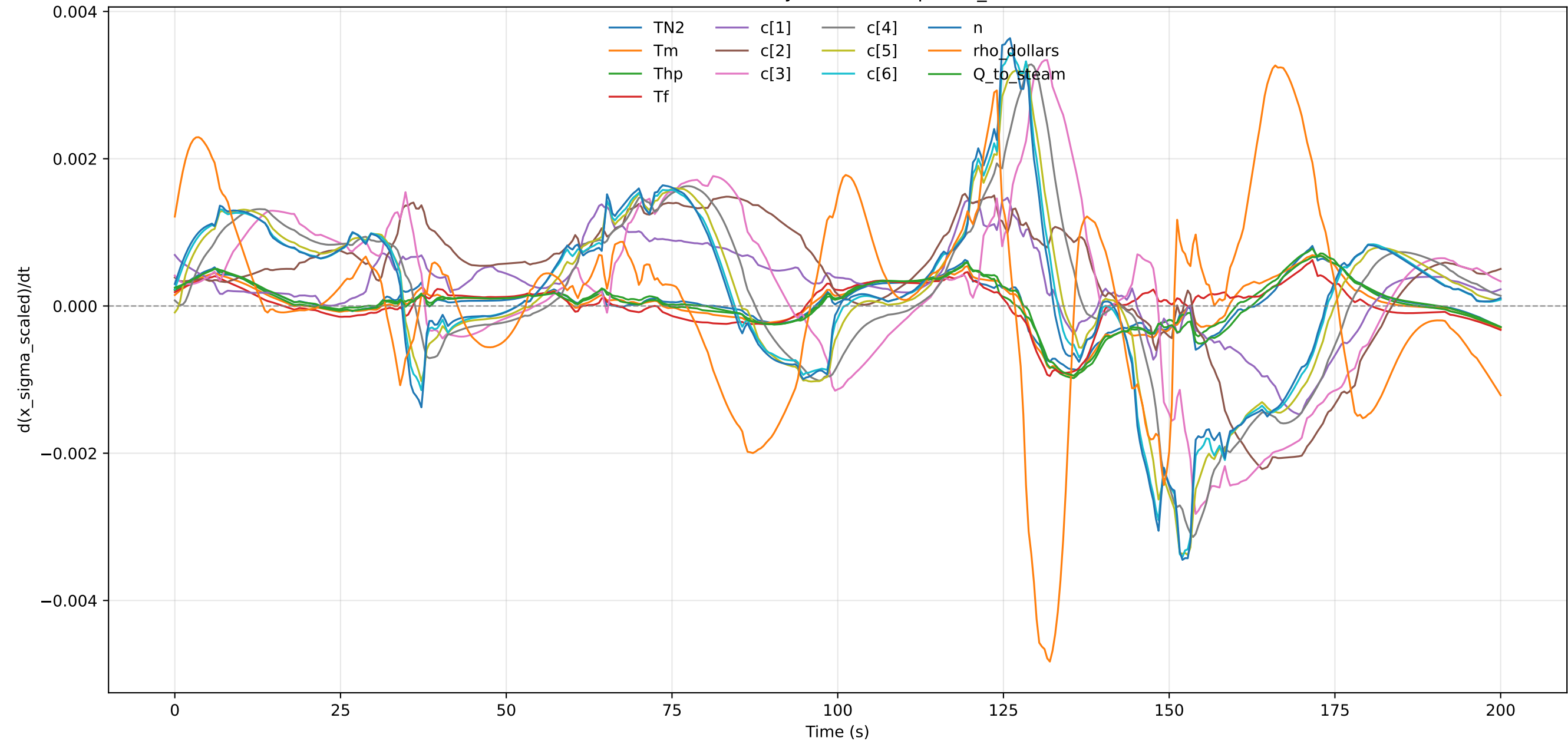
Scaled Uncertainty Derivative - profile_000006
