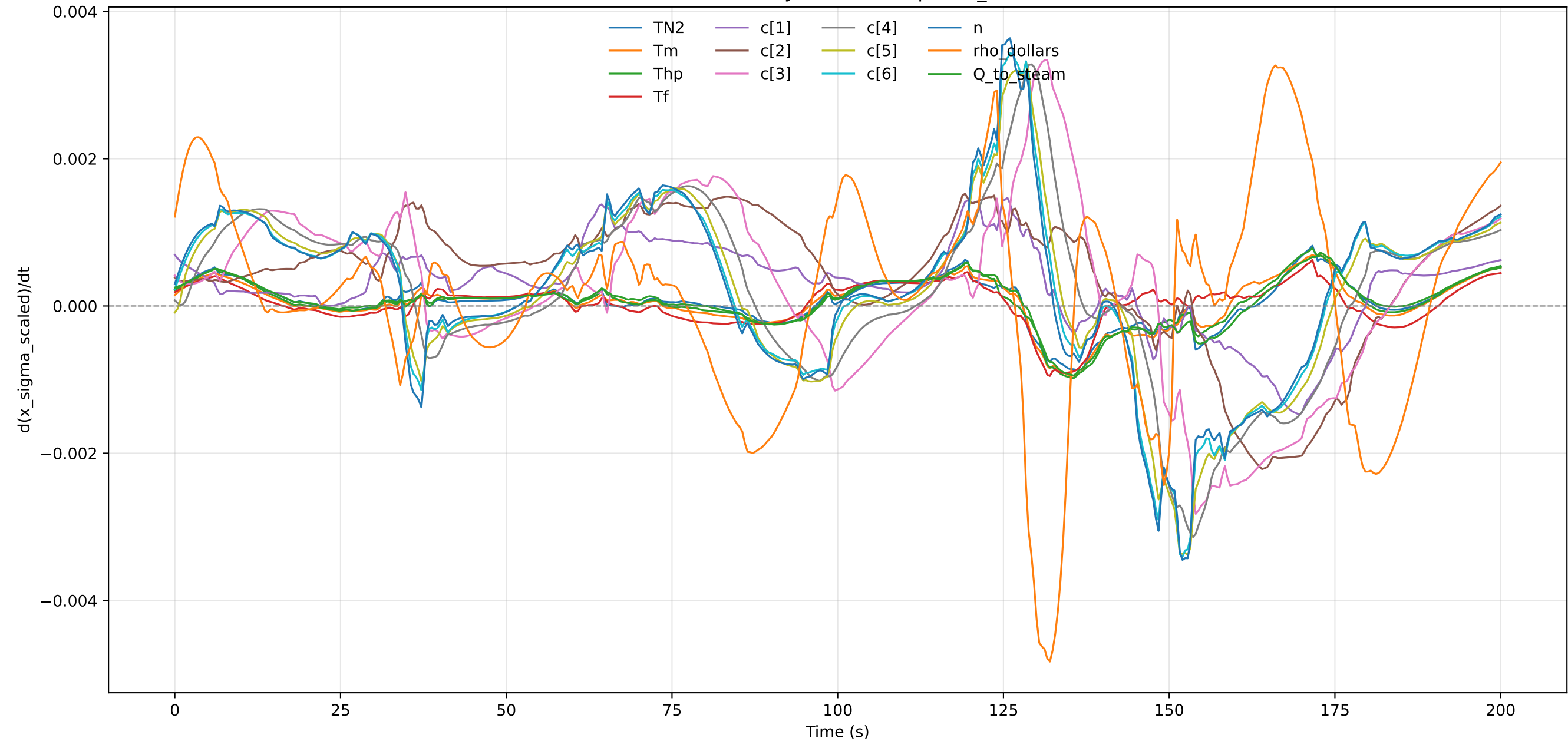
Scaled Uncertainty Derivative - profile_000021
