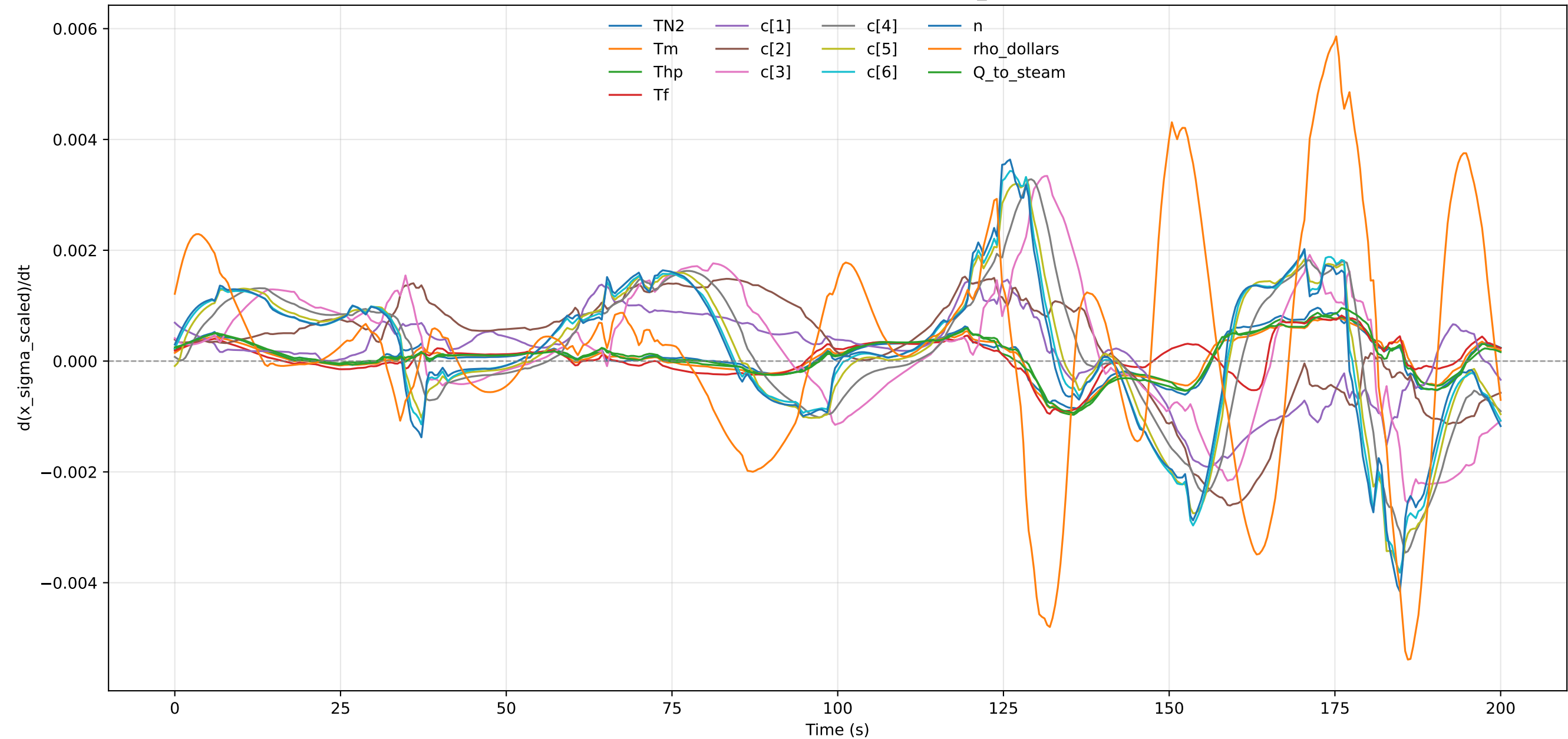
Scaled Uncertainty Derivative - profile_000011
