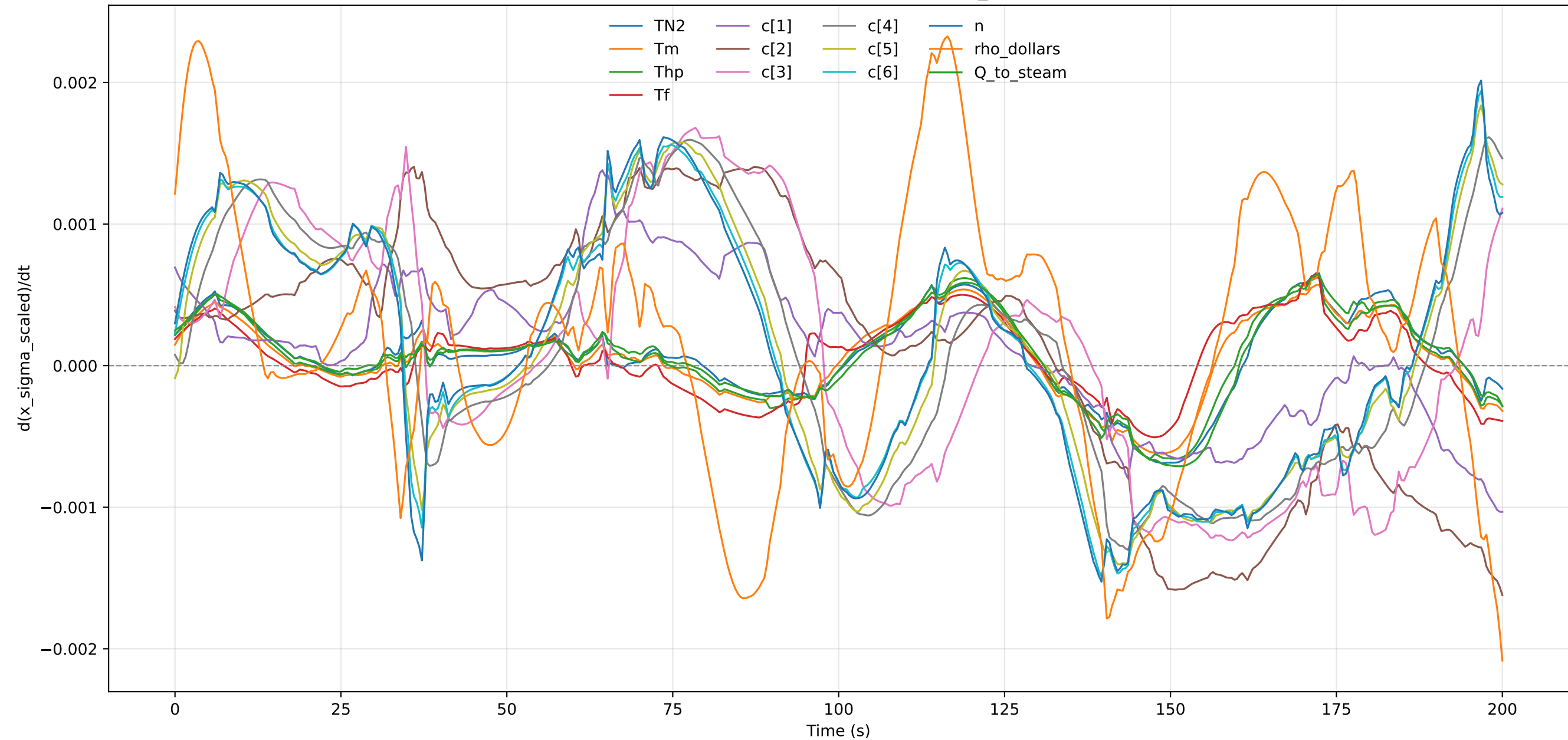
Scaled Uncertainty Derivative - profile_000016
