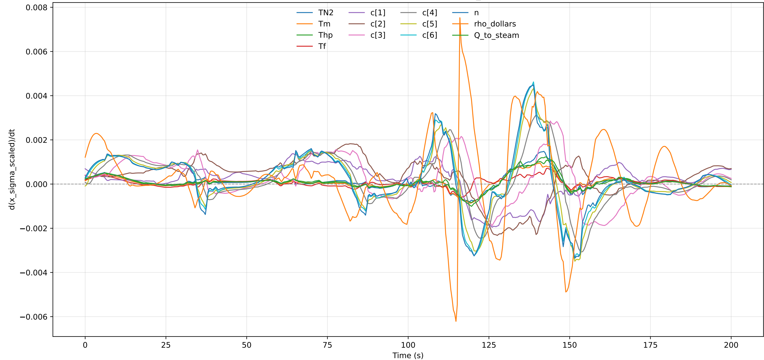
Scaled Uncertainty Derivative - profile_000007
