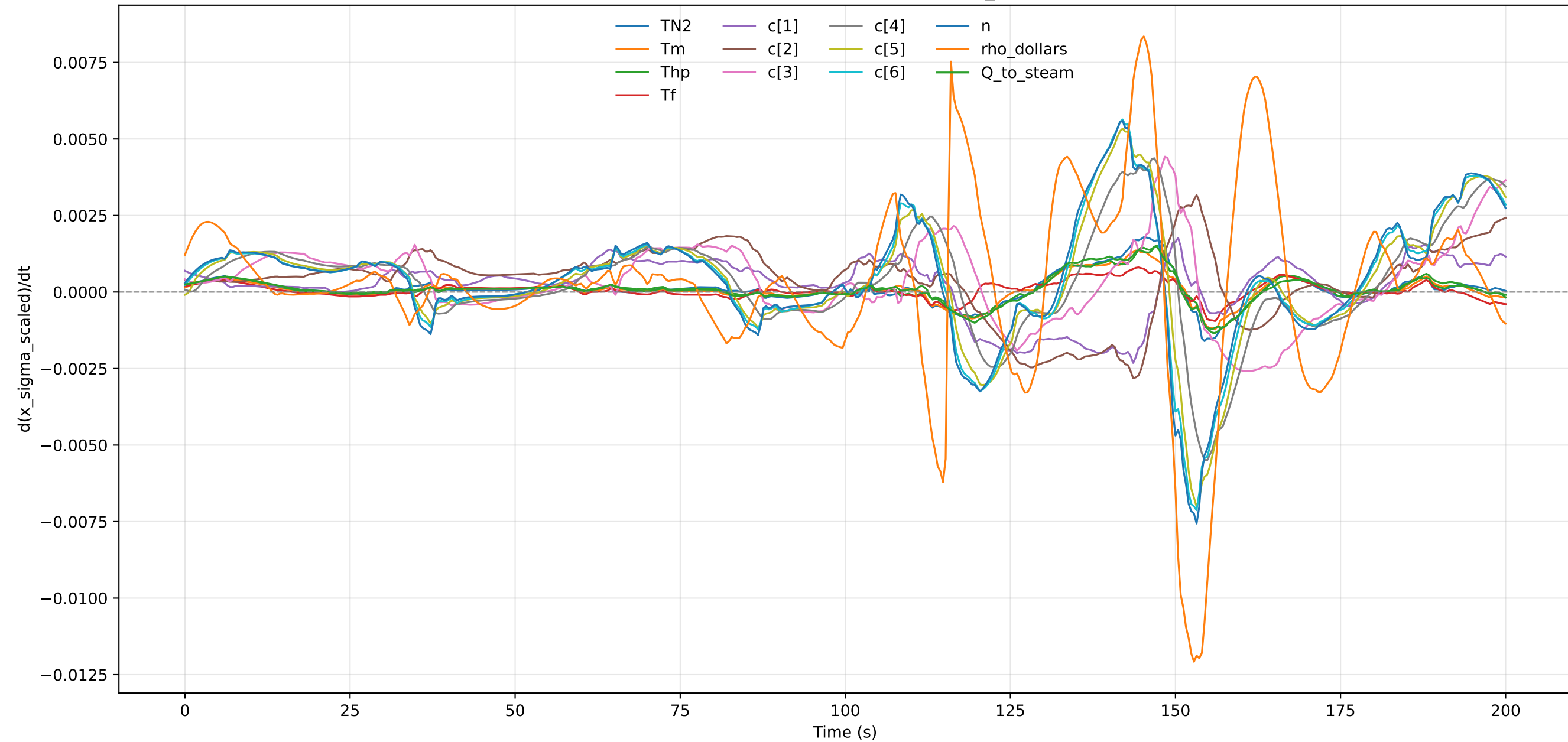
Scaled Uncertainty Derivative - profile_000026
