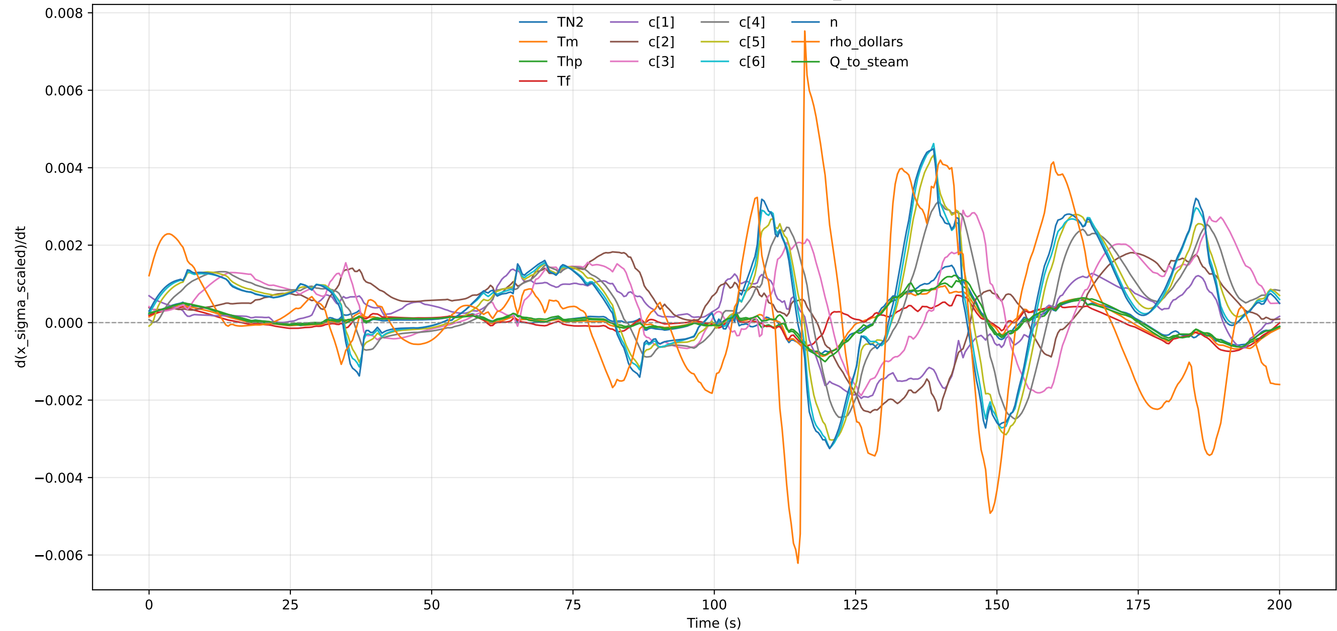
Scaled Uncertainty Derivative - profile_000024
