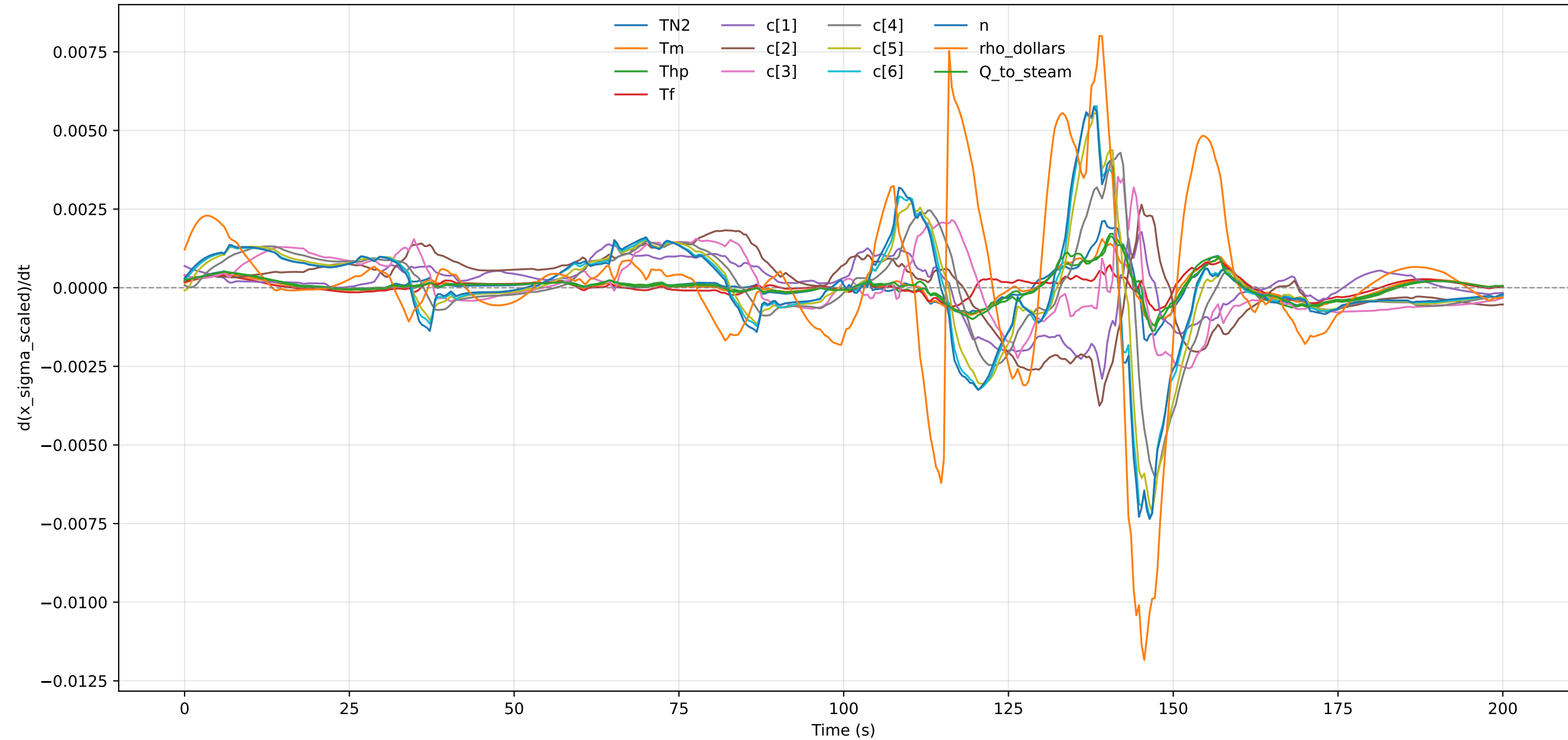
Scaled Uncertainty Derivative - profile_000014
