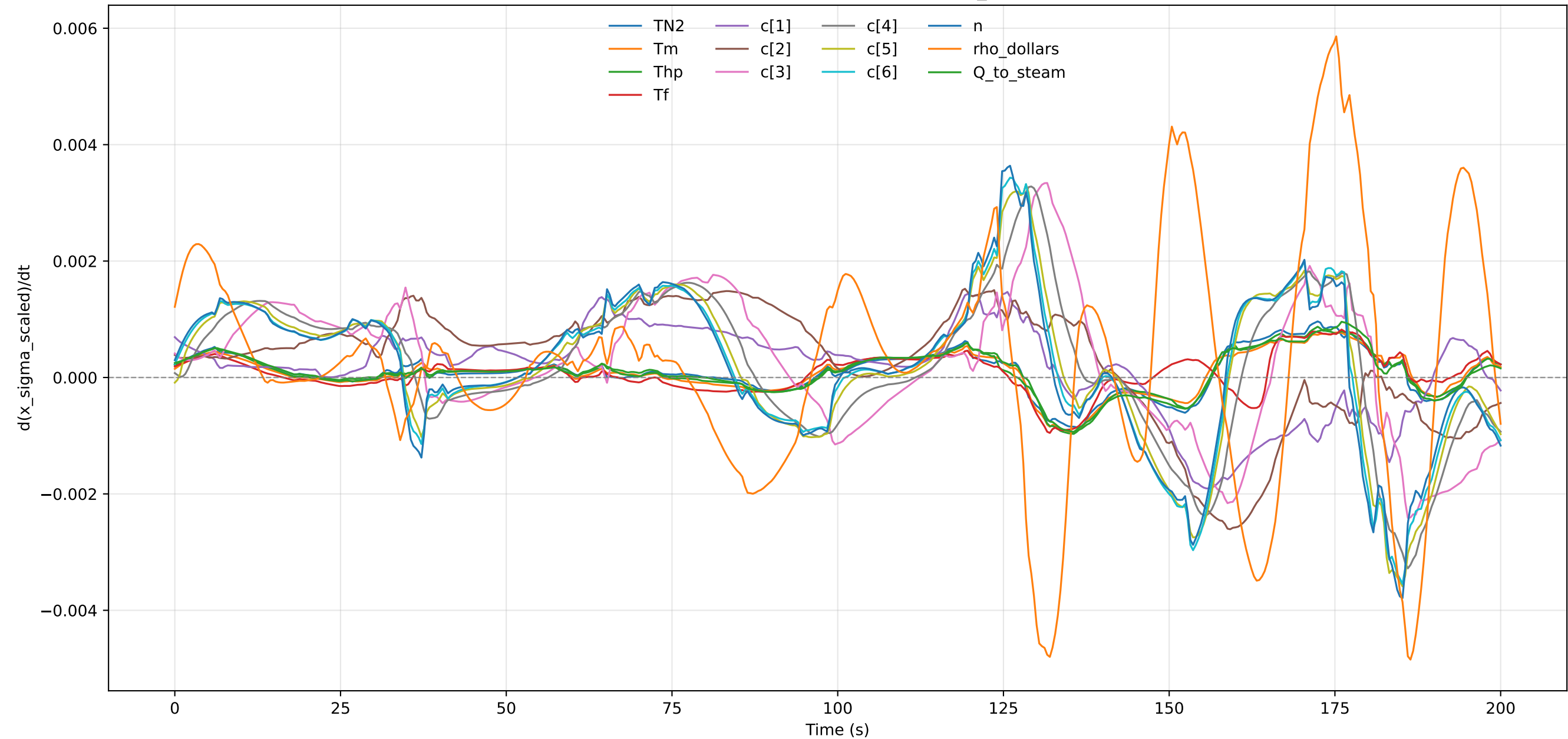
Scaled Uncertainty Derivative - profile_000012
