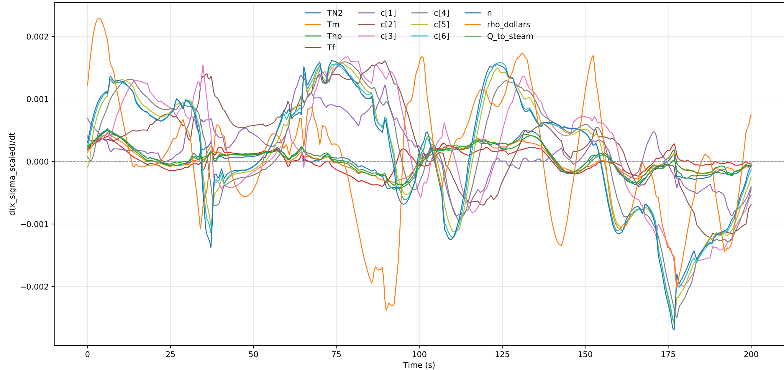
Scaled Uncertainty Derivative - profile_000000
