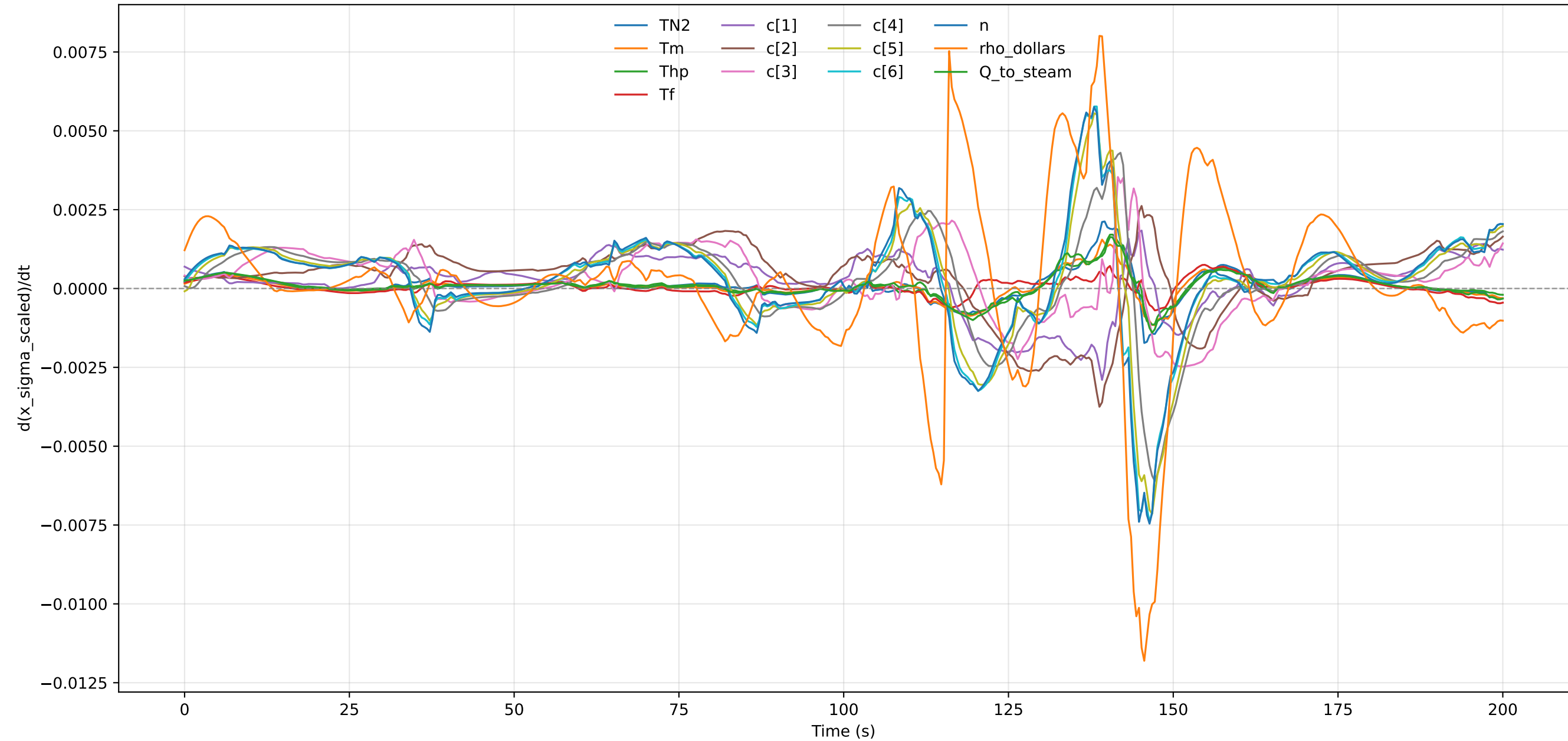
Scaled Uncertainty Derivative - profile_000002
