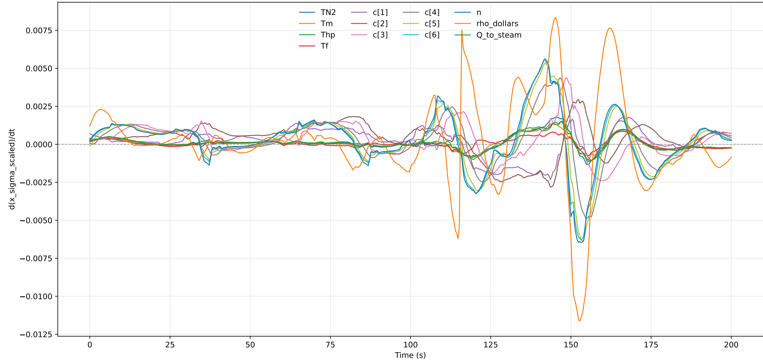
Scaled Uncertainty Derivative - profile_000008
