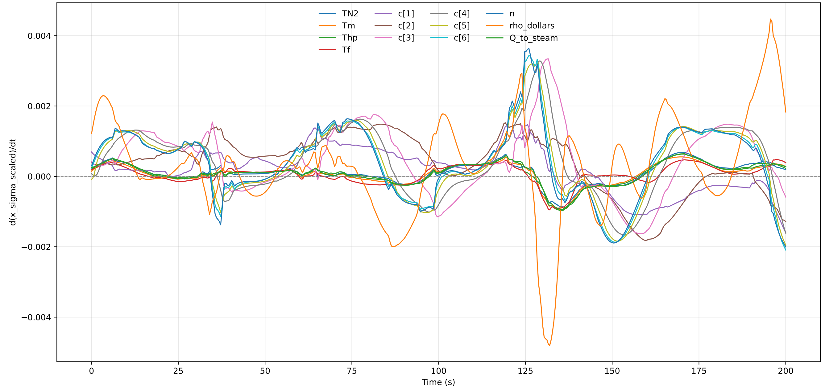
Scaled Uncertainty Derivative - profile_000019
