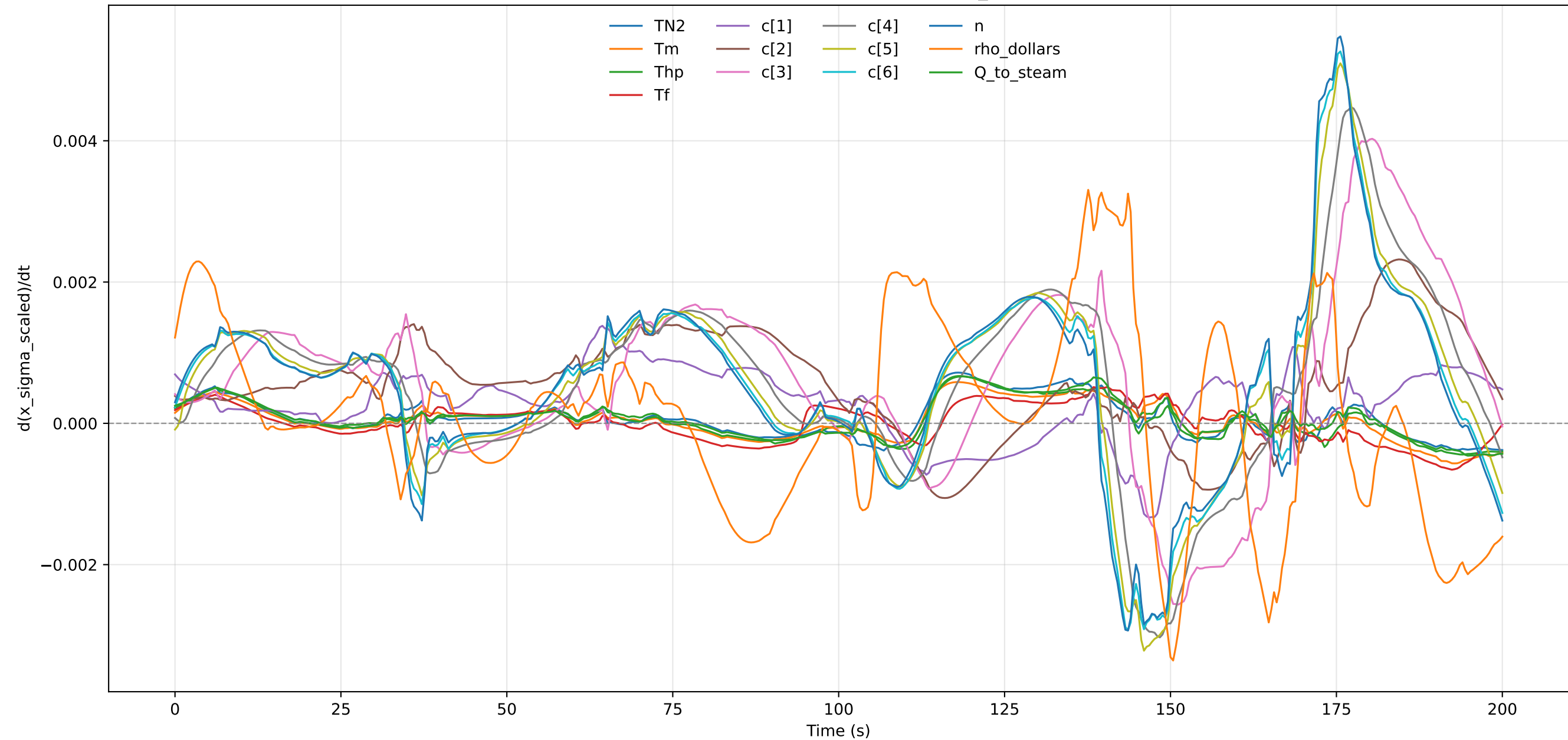
Scaled Uncertainty Derivative - profile_000017
