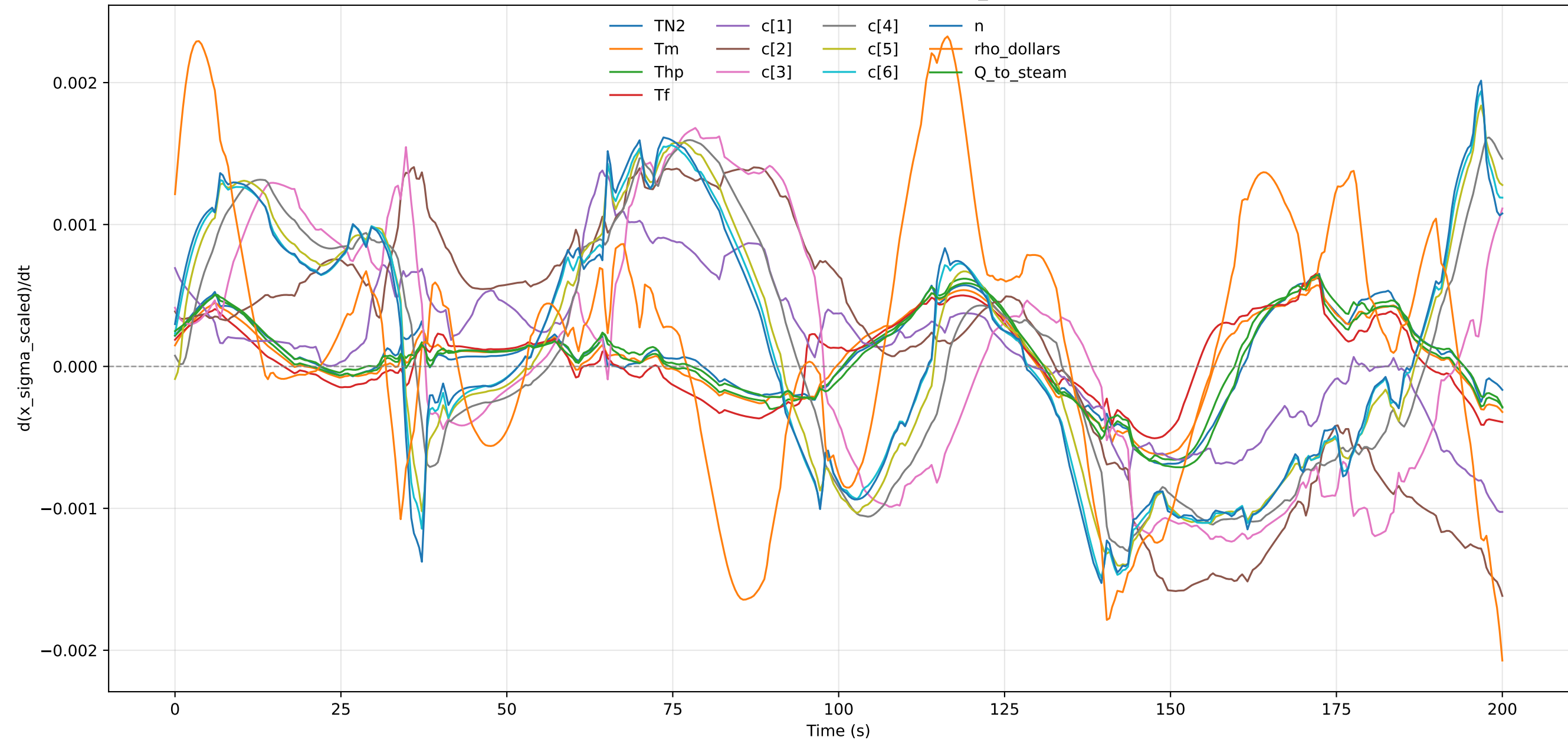
Scaled Uncertainty Derivative - profile_000015
