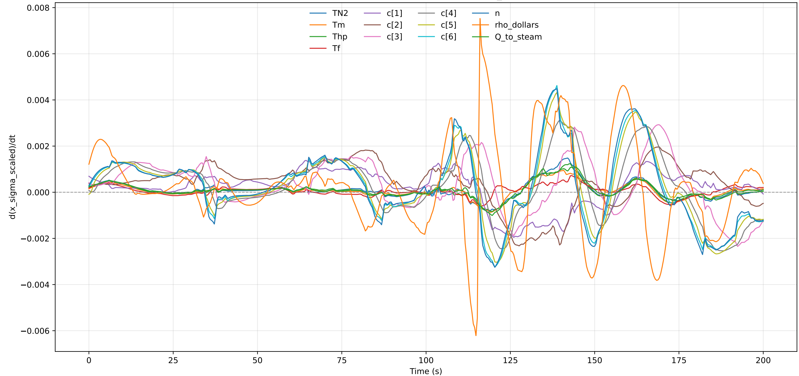
Scaled Uncertainty Derivative - profile_000023
