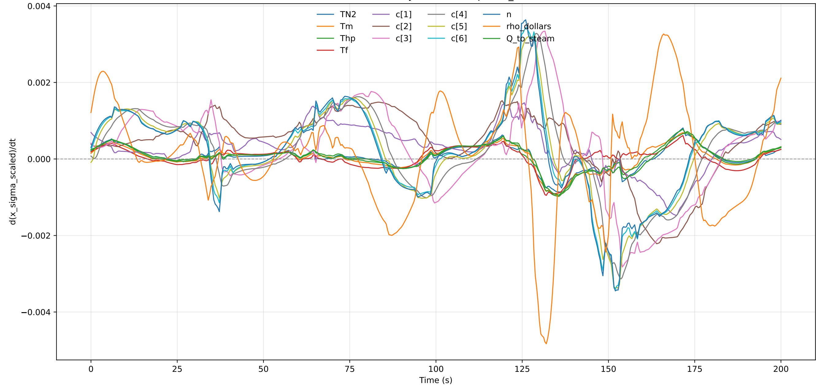
Scaled Uncertainty Derivative - profile_000022
