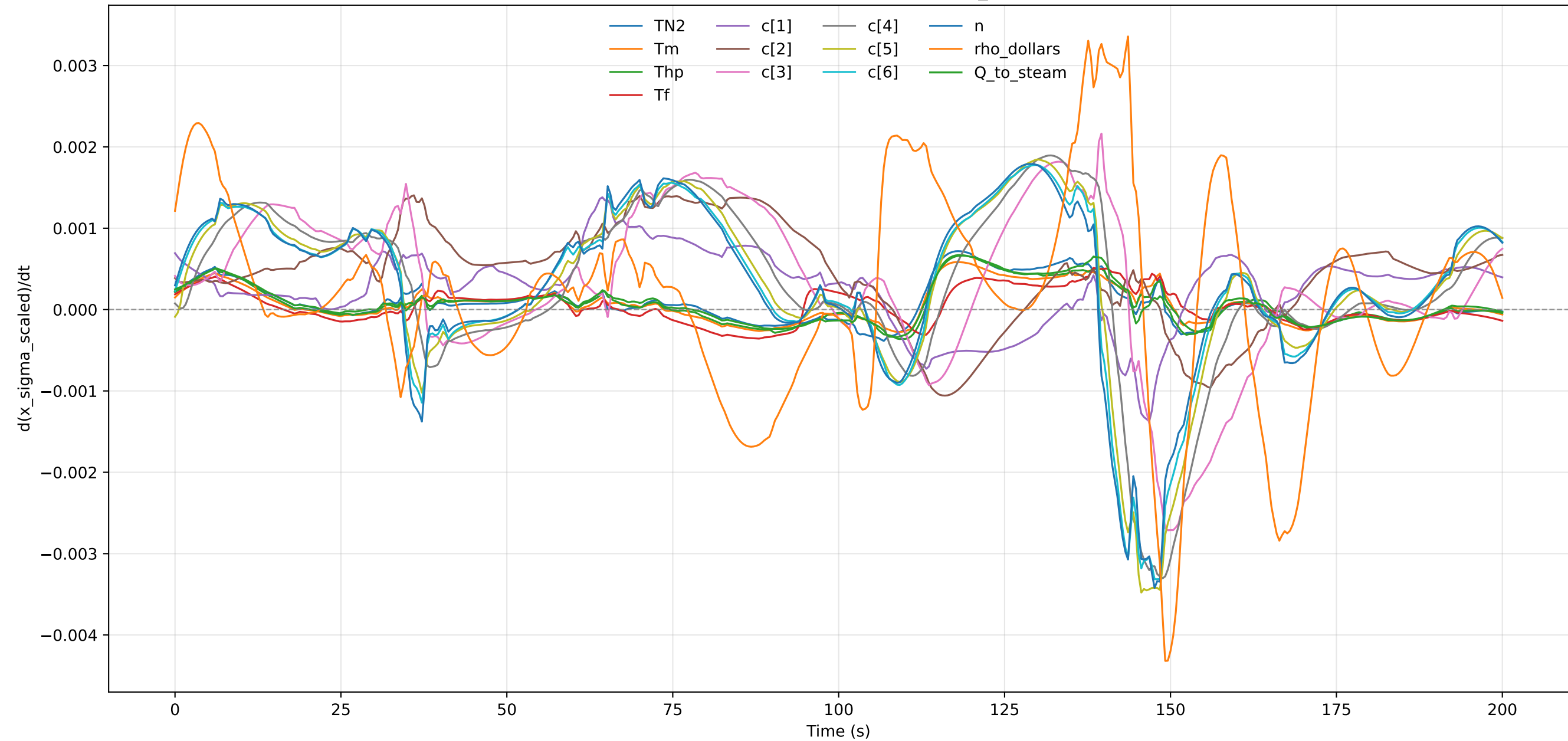
Scaled Uncertainty Derivative - profile_000018
