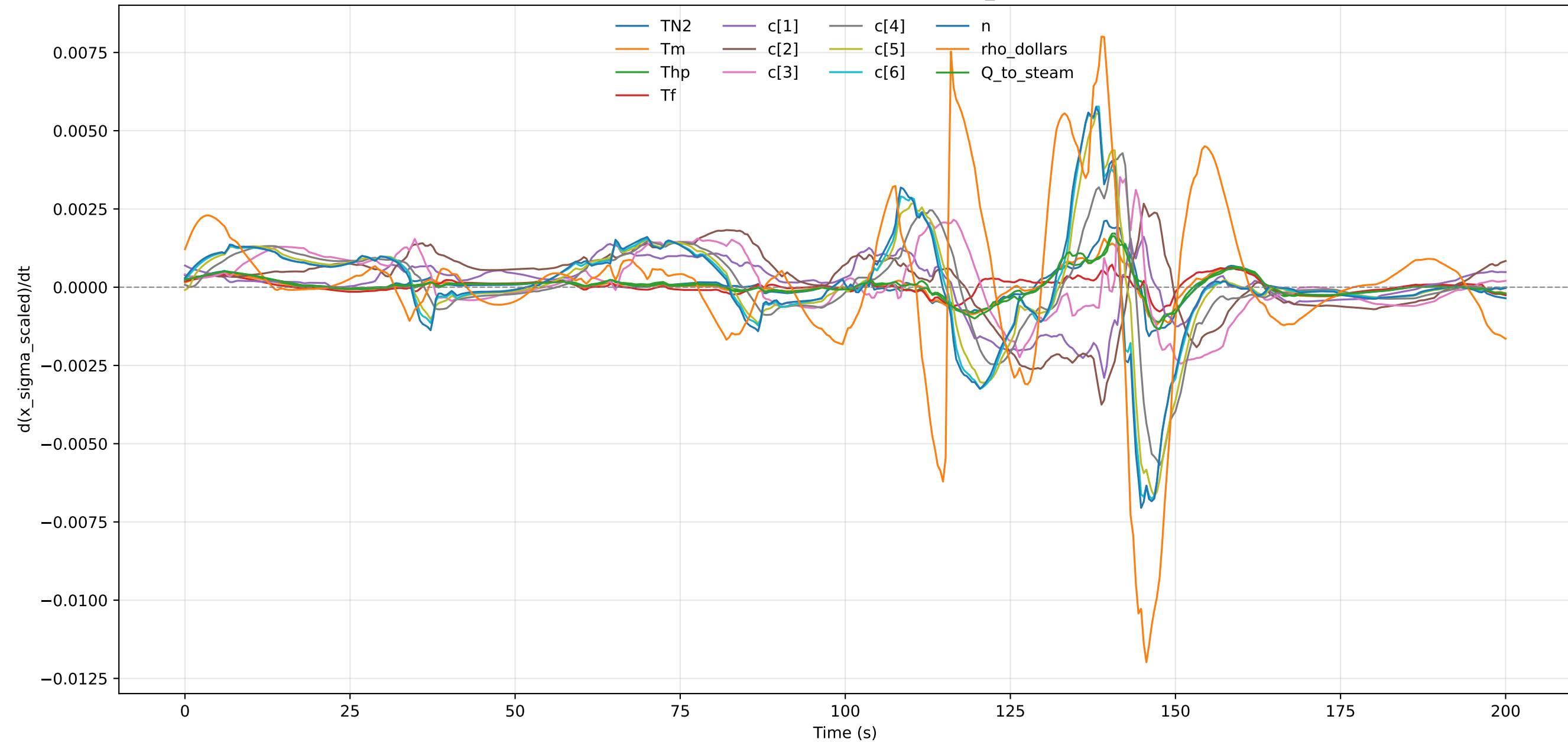
Scaled Uncertainty Derivative - profile_000013
