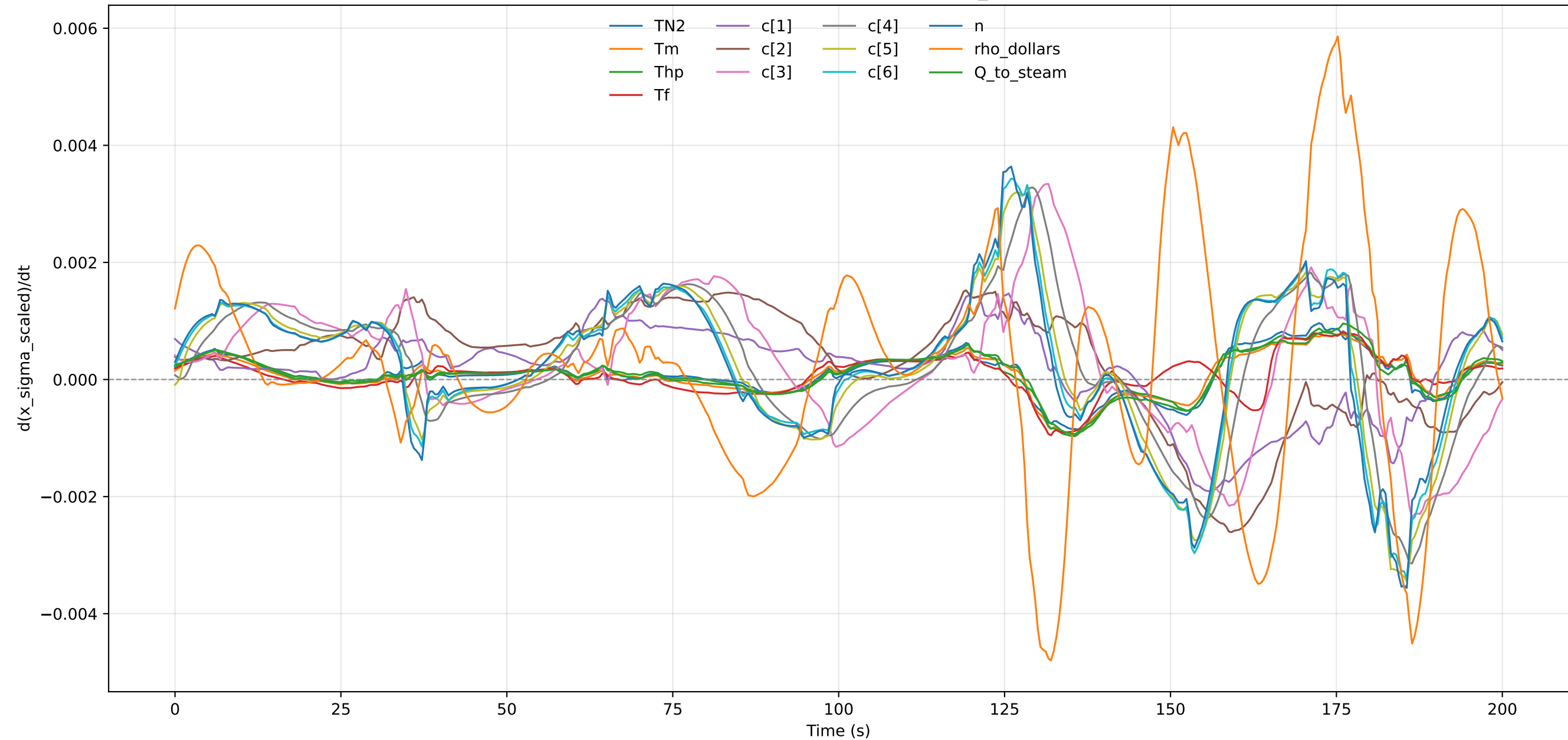
Scaled Uncertainty Derivative - profile_000001
