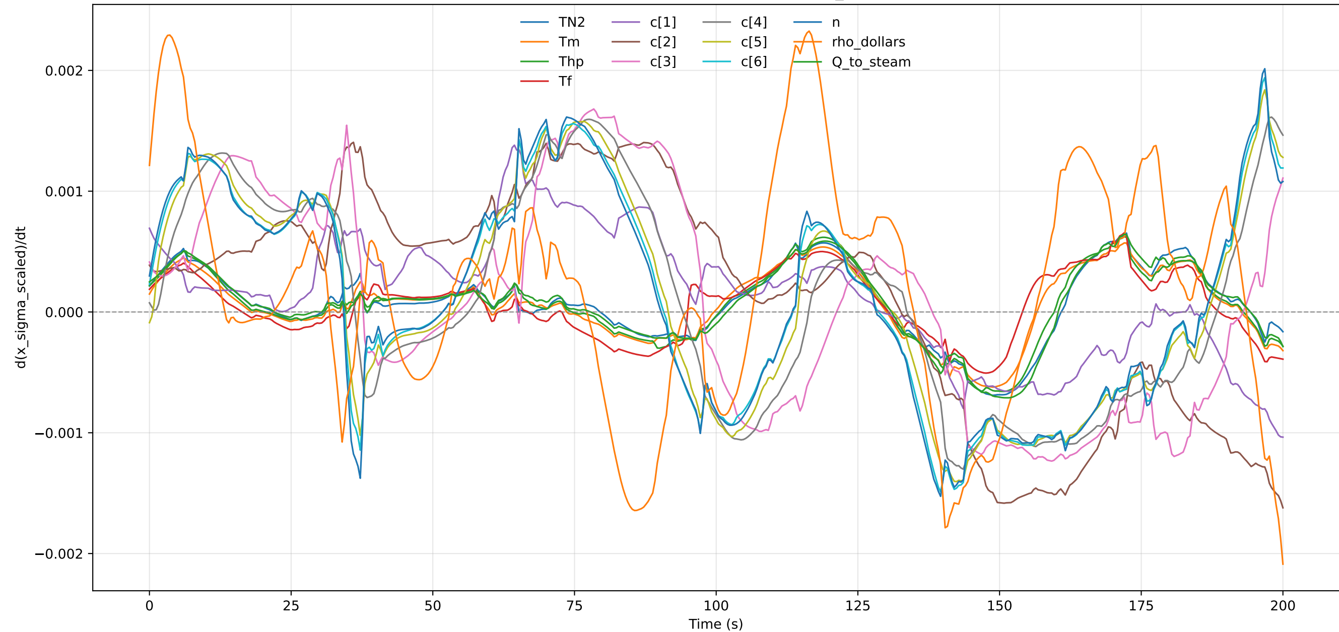
Scaled Uncertainty Derivative - profile_000003
