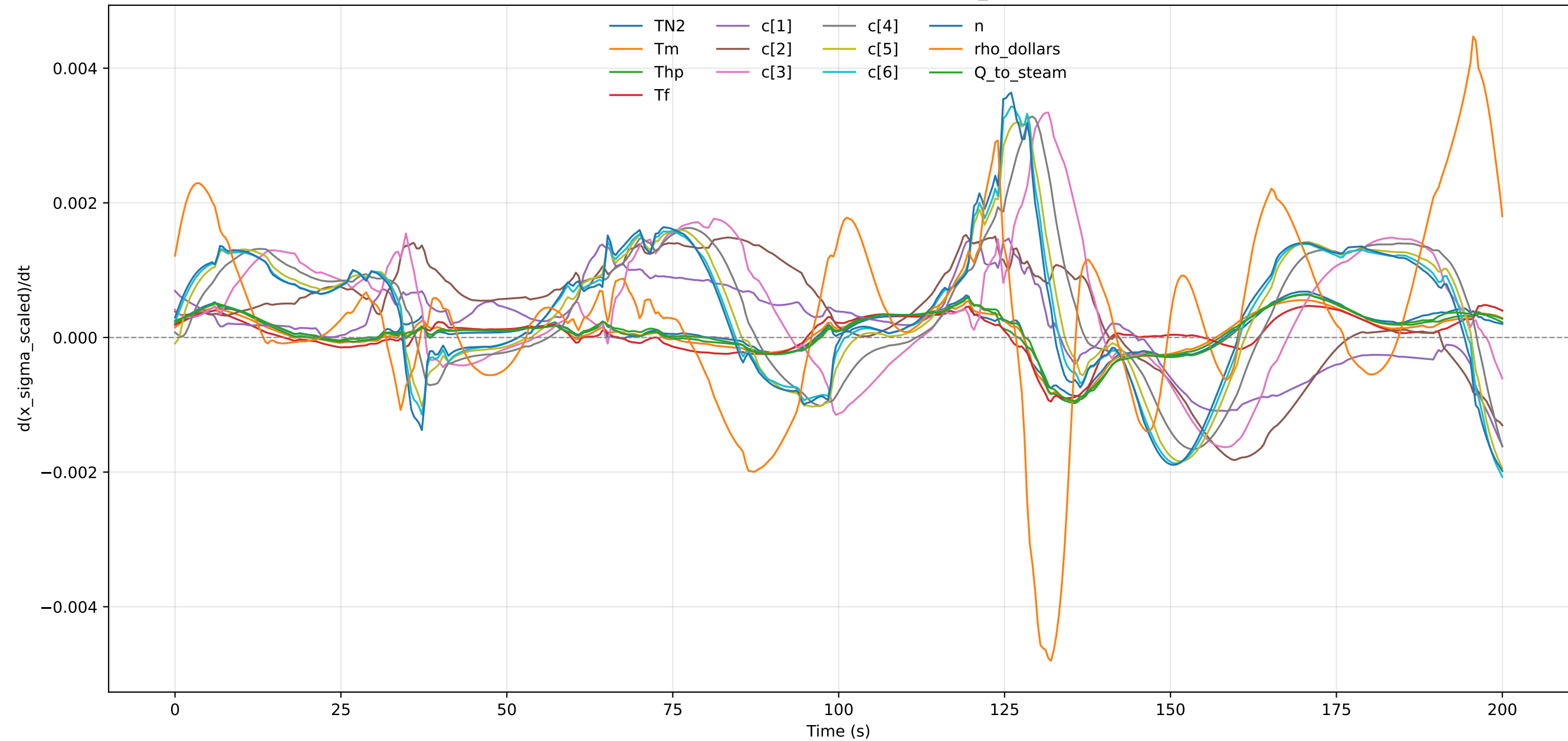
Scaled Uncertainty Derivative - profile_000005
