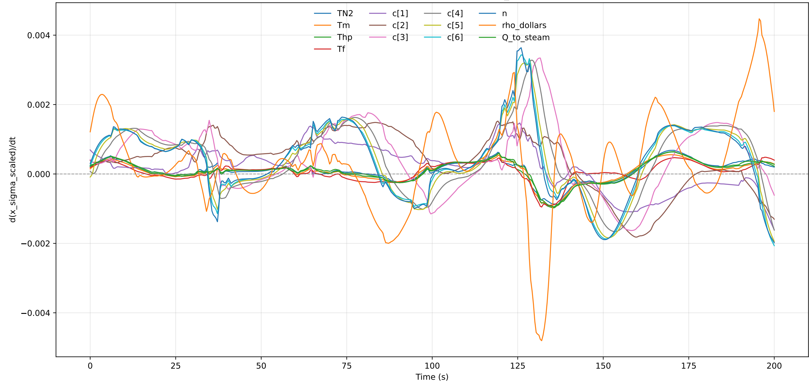
Scaled Uncertainty Derivative - profile_000020
