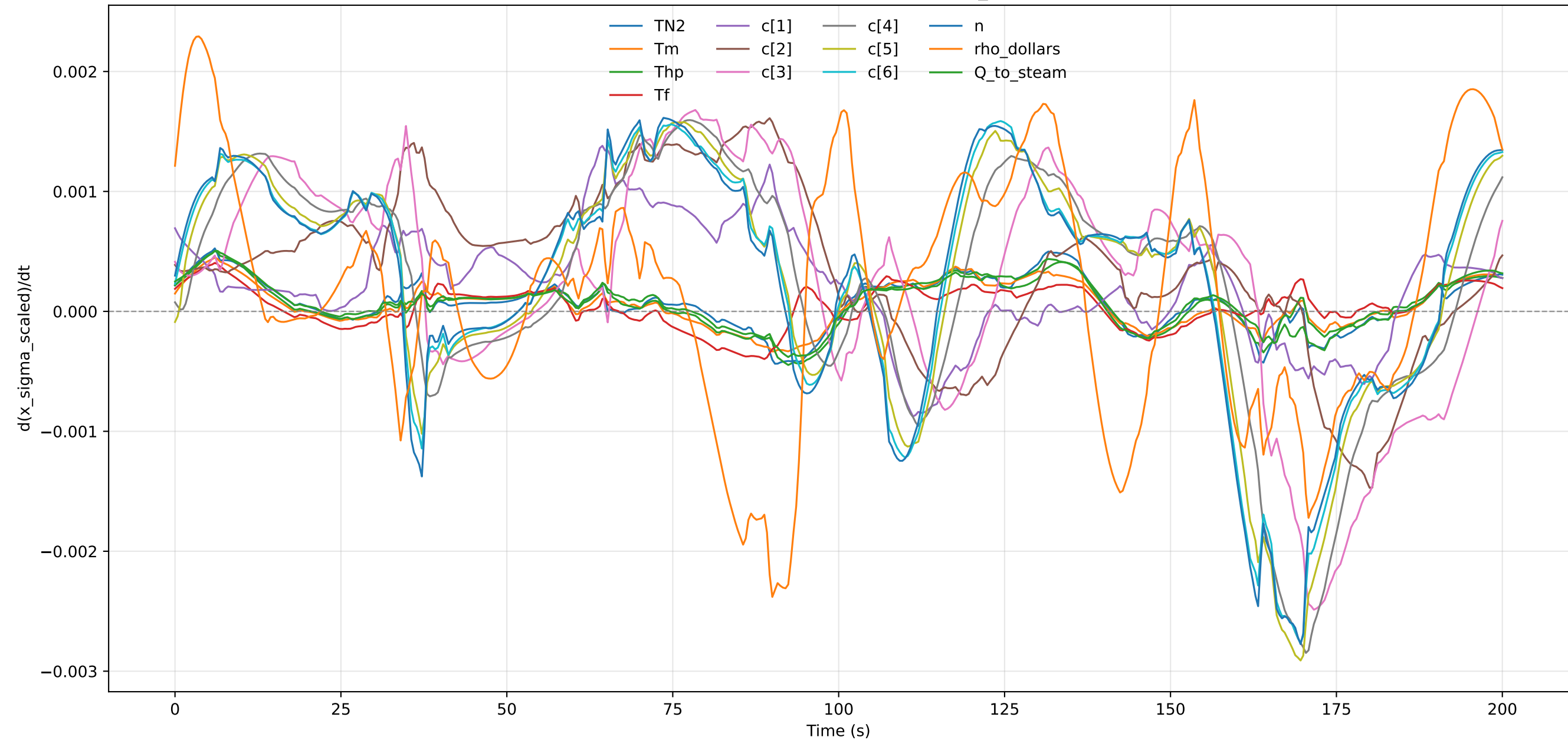
Scaled Uncertainty Derivative - profile_000010
