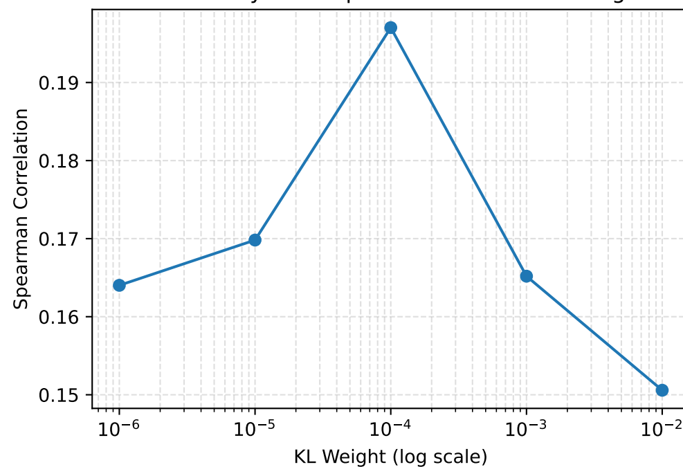
Uncertainty-Error Spearman Corr vs KL Weight
