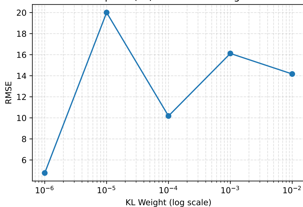
Output 2 (TF) RMSE vs KL Weight
