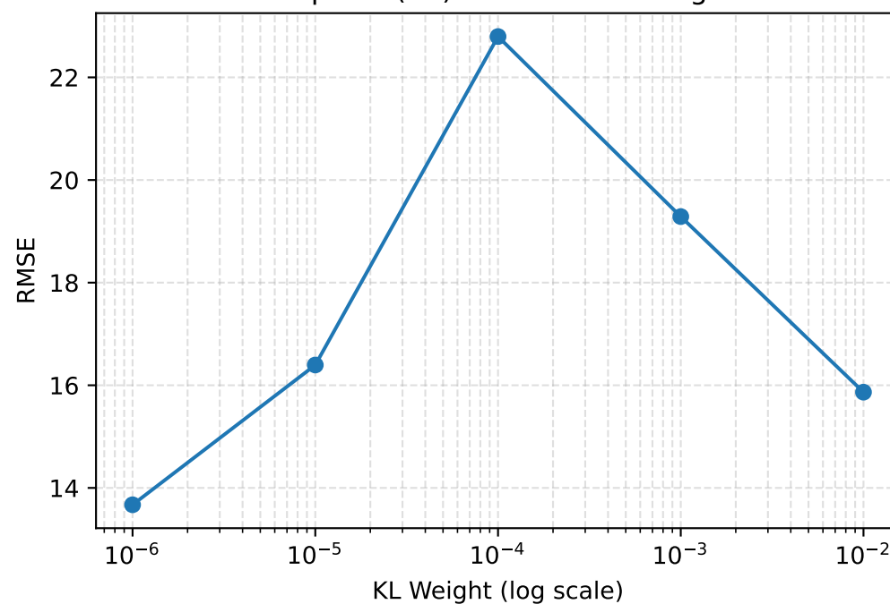
Output 1 (TS) RMSE vs KL Weight
