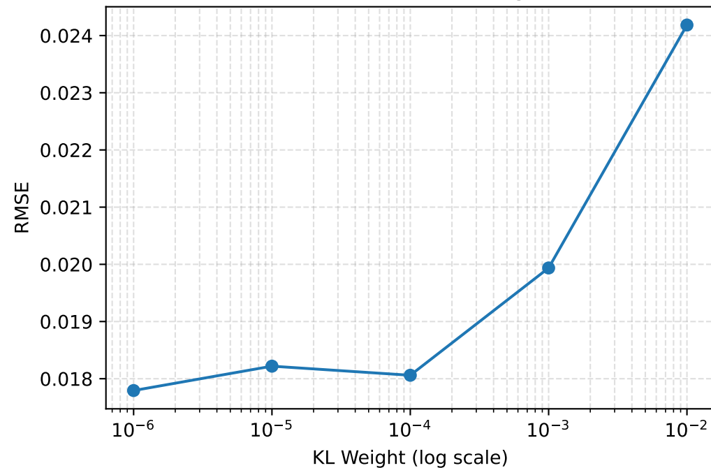
Solar RMSE vs KL Weight
