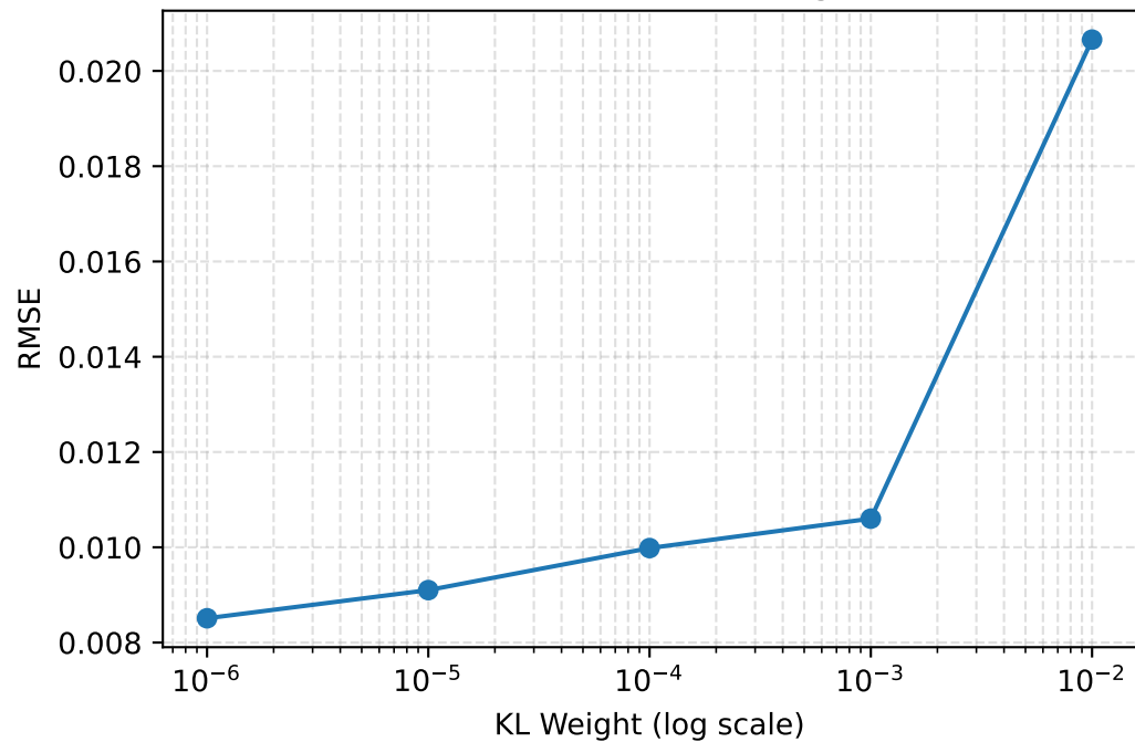
Wind RMSE vs KL Weight
