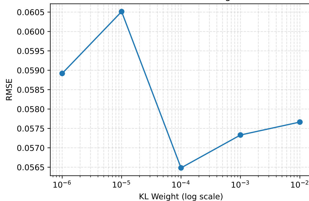
Solar RMSE vs KL Weight
