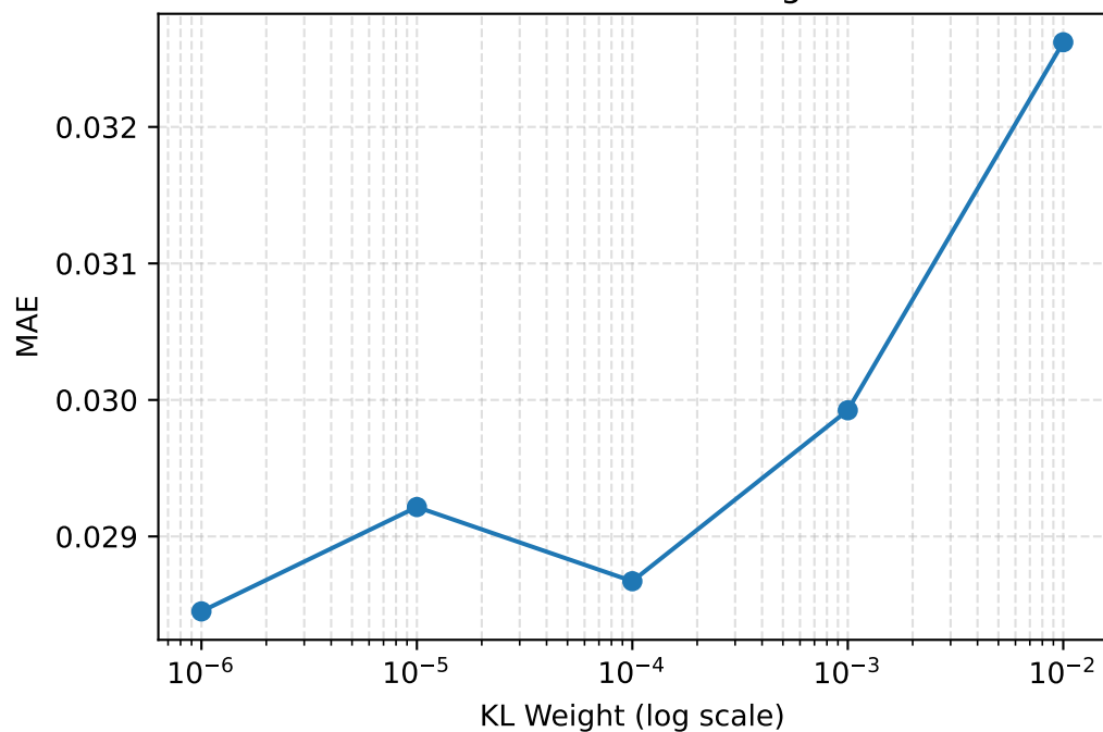
Solar MAE vs KL Weight
