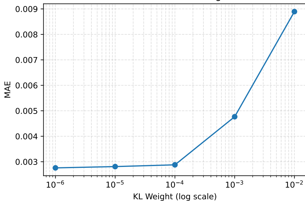
Wind MAE vs KL Weight
