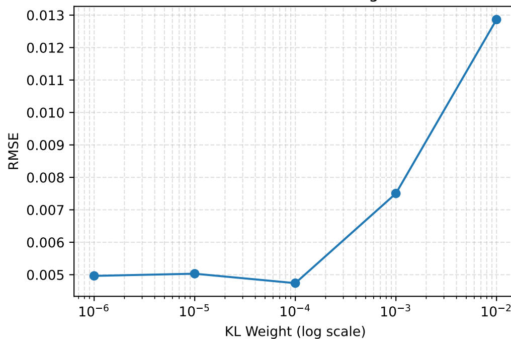
Wind RMSE vs KL Weight
