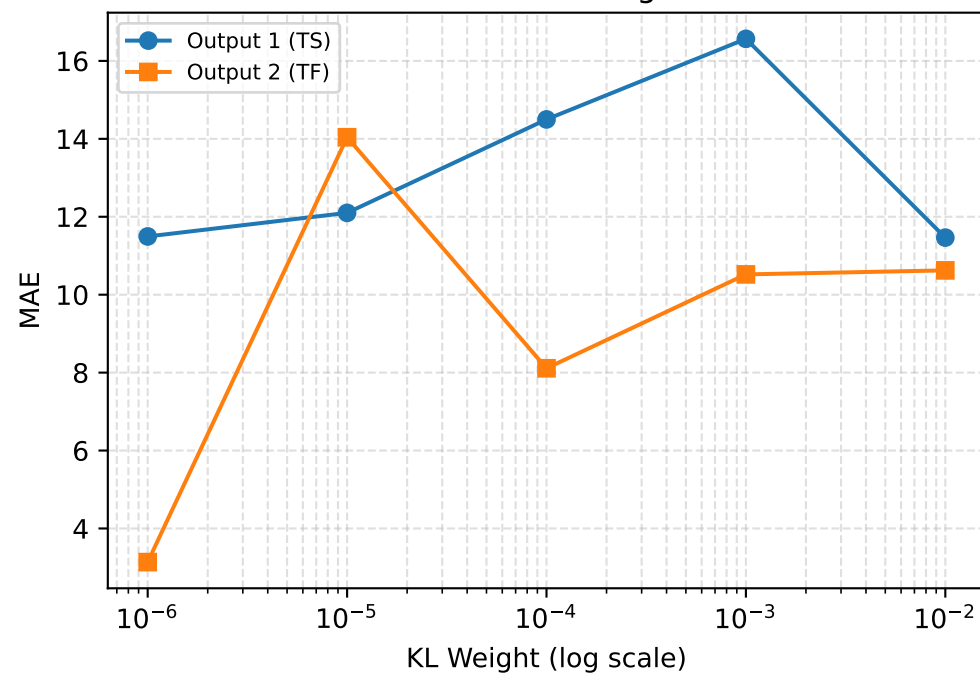
MAE vs KL Weight
