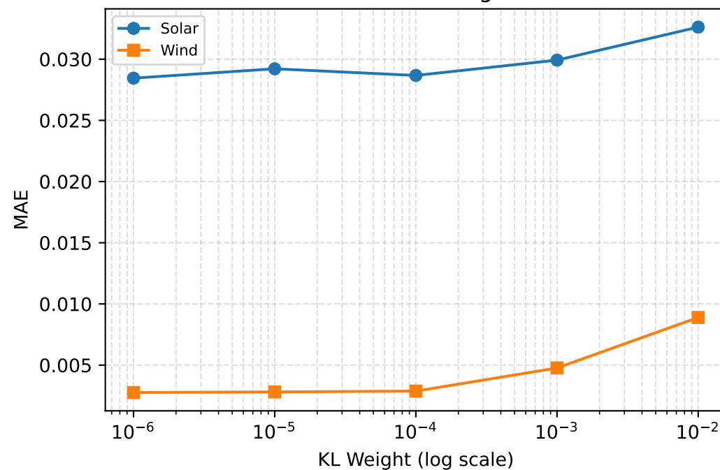
MAE vs KL Weight
