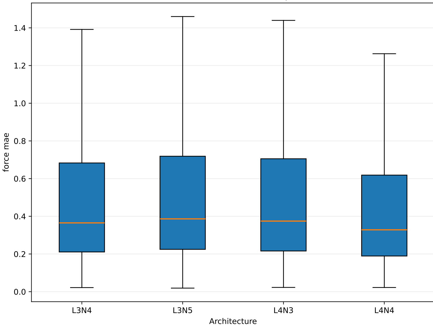
Force Mae by architecture Values above each run mean + 5 sample SD removed
