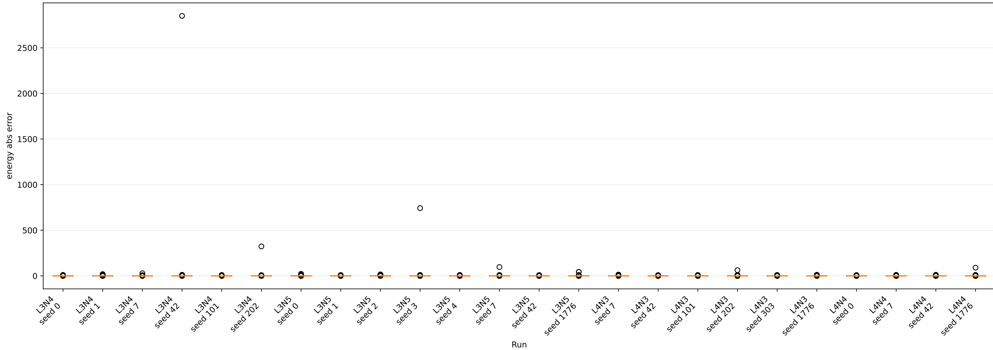
Energy Abs Error by run
