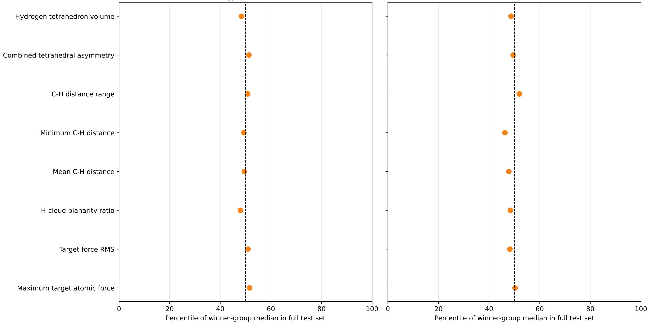
All robust energy-error wins (N=3,591)
