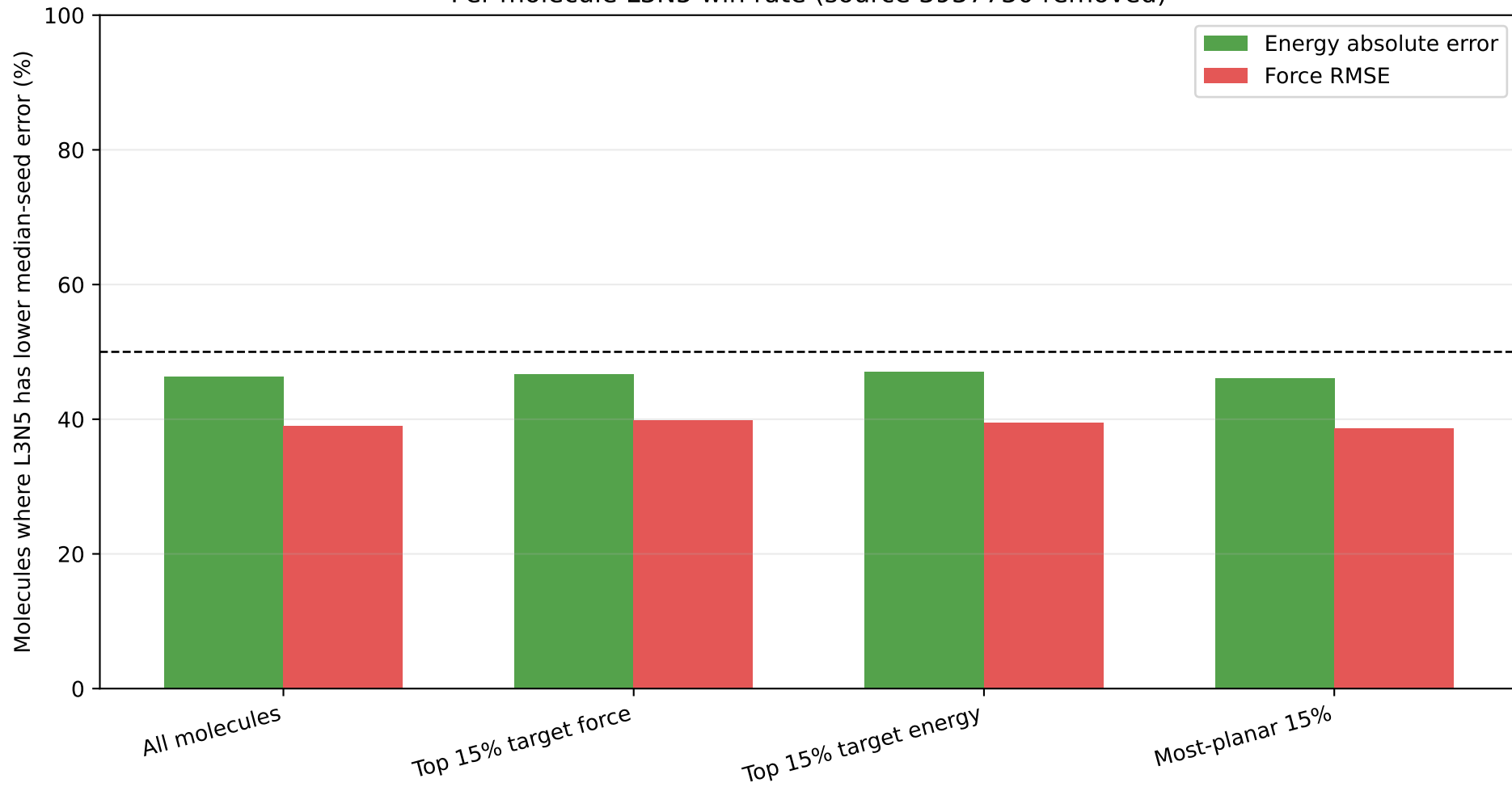
Per-molecule L3N5 win rate (source 3937730 removed)
