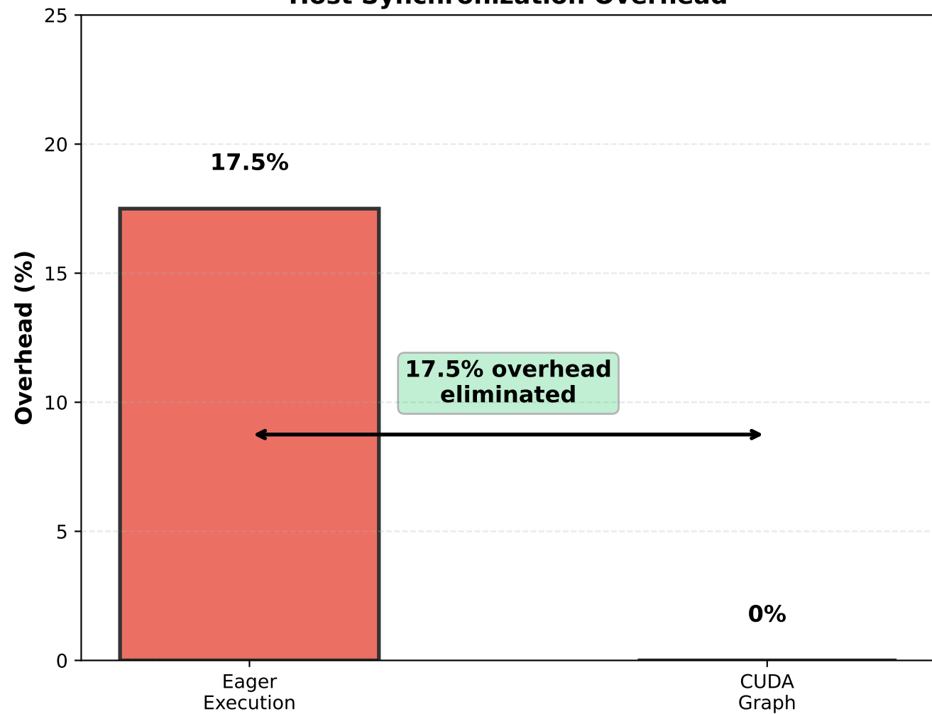
Host Synchronization Overhead
