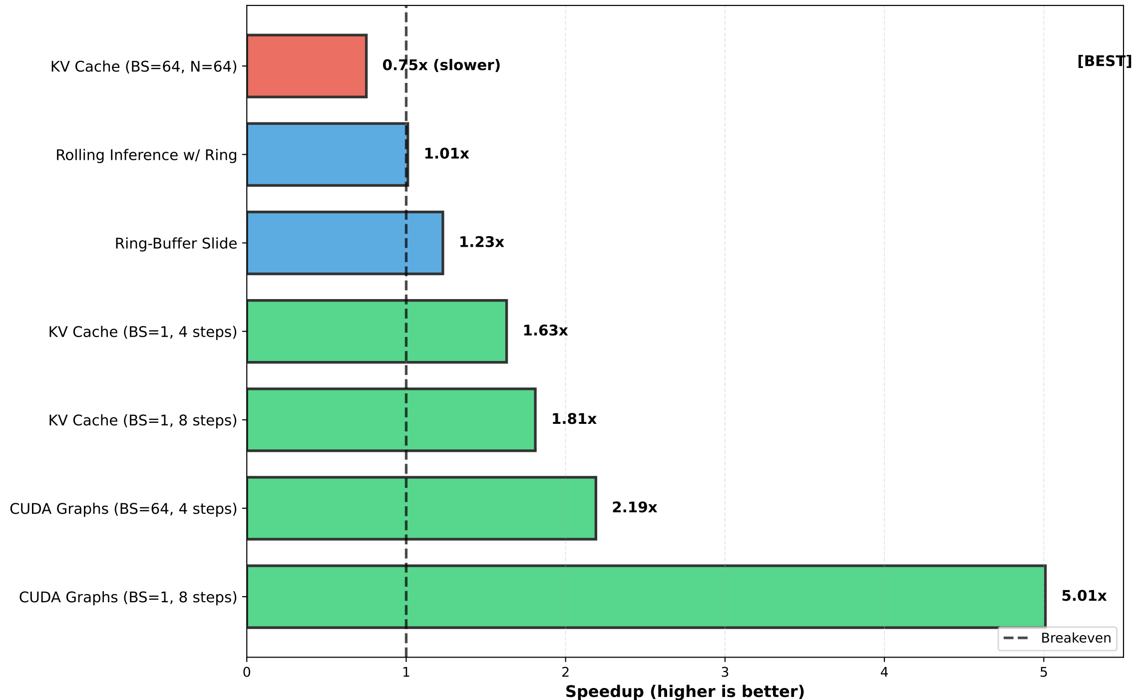
Optimization Leaderboard: Speedup Comparison
