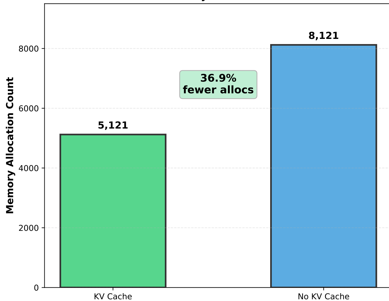
Memory Allocations
