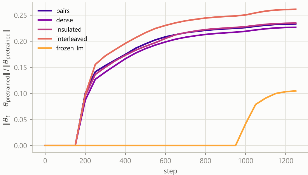
Drift of the text expert from the pretrained language model
