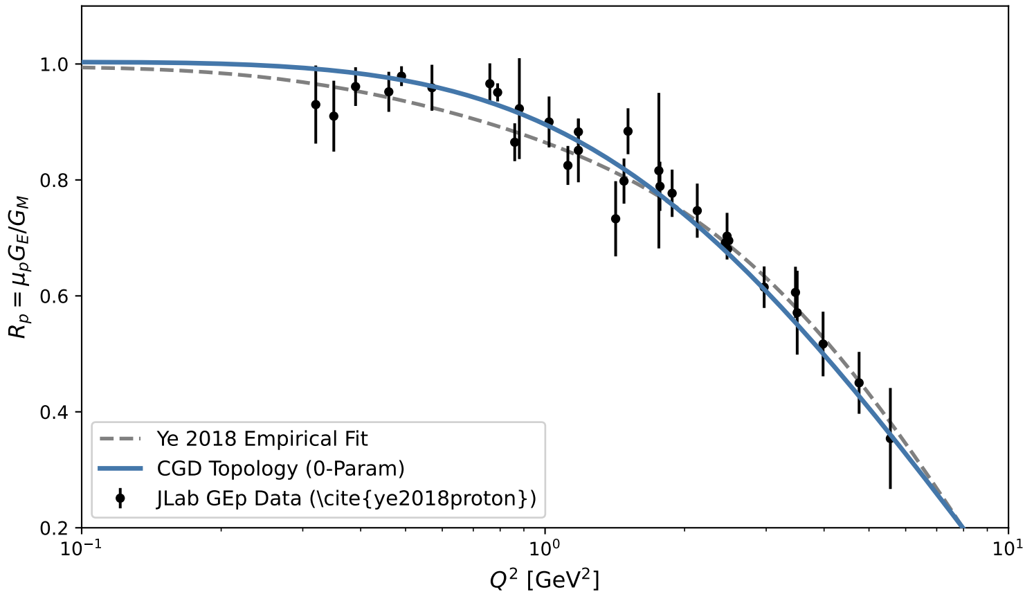
Proton Core Form Factor: Empirical Baseline vs. CGD Topology
