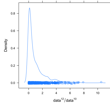
(b) Densityplot
