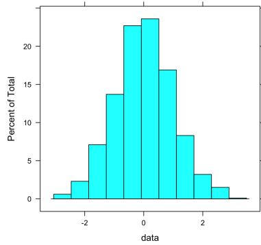
(a) Histogram
