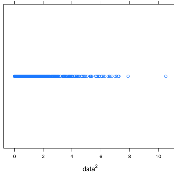
(c) Stripplot
